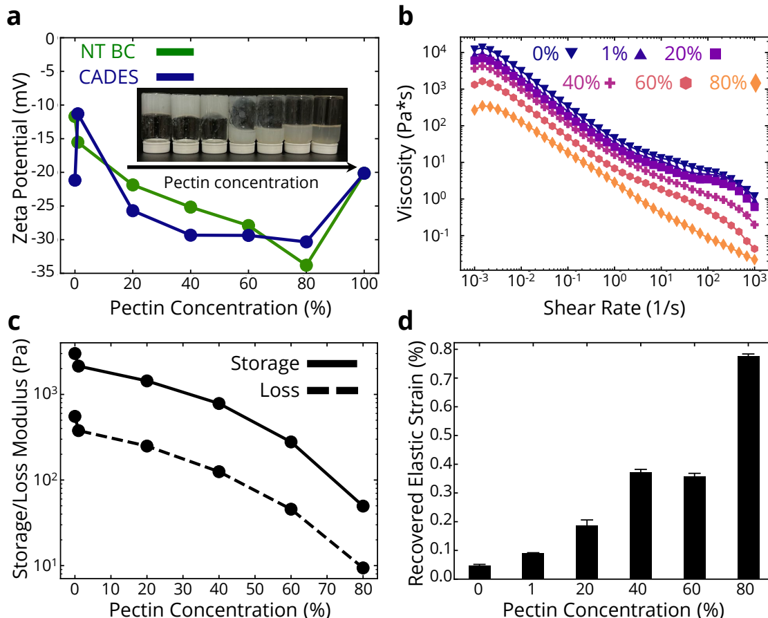
Fig. 3 Effects of Adding Pectin on Colloidal Properties. (a), Zeta potential measurements of non-treated and CADES BC dispersions with varying amounts of pectin added. Viscosity measurements (b) and storage/loss moduli at \sim 5 rad/s (c) of CADES BC/pectin dispersions (d), Recovered elastic strain percentage of CADES BC/pectin dispersions.
