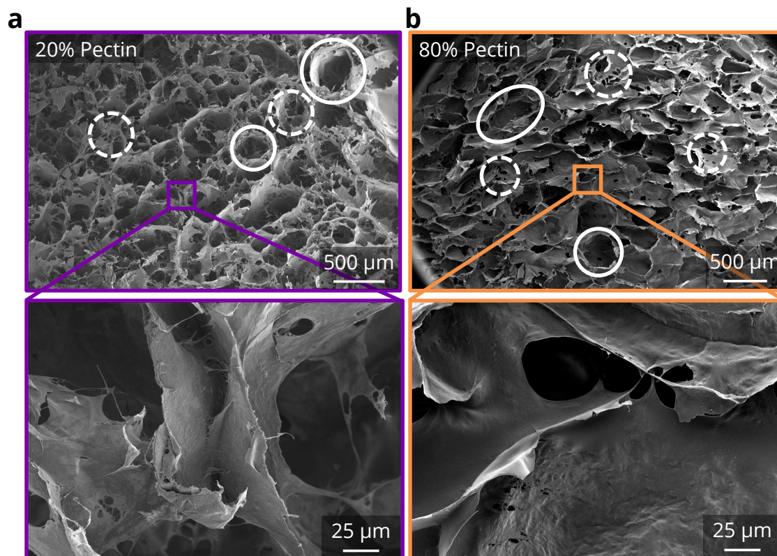
Fig. 5 Effects of Adding Pectin on Morphological Properties. SEM images of a CADES BC foam with (a) 20% pectin and (b) 80% pectin at 30x (top row) and 500x (bottom row) magnifications. Solid circles indicate cells in the foams, dashed circles indicate holes in the matrix.
