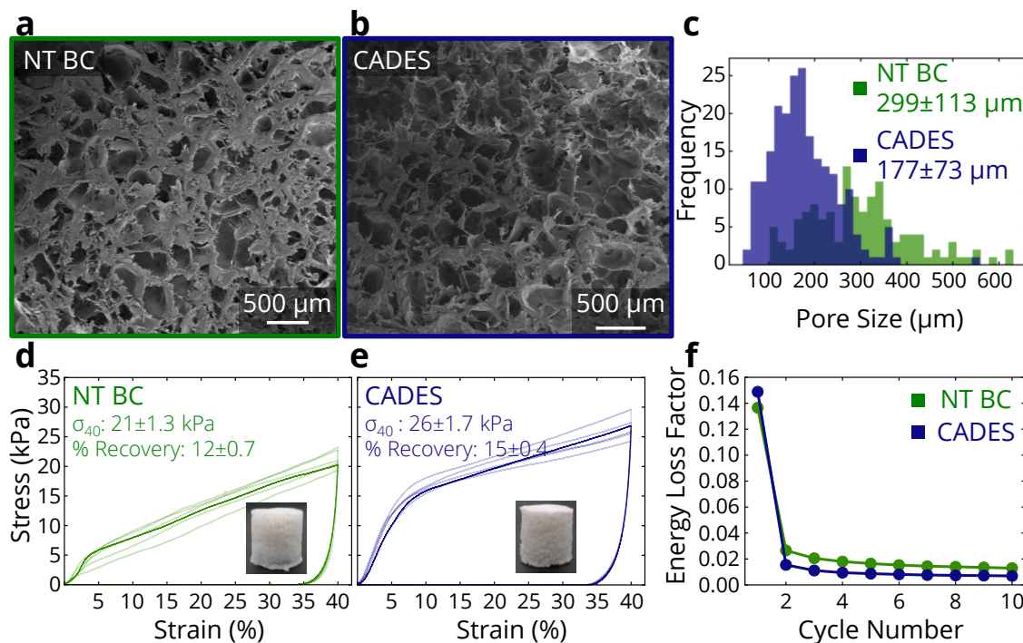
Fig. 2 Morphological and mechanical effects of DES treatment on BC foams. SEM of non-treated BC (a) and CADES BC (b) foams. (c), Distribution of pore sizes for non-treated and CADES BC foams. Compression tests of non-treated (d) and CADES (e) BC foams. (f), Energy loss factors from cyclic testing of non-treated and CADES BC foams.
