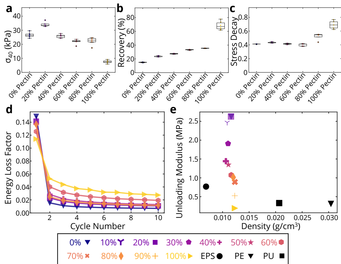
Fig. 6 Effects of Adding Pectin on Mechanical Properties. Compressive strength (a) and recovery percentage (b) from 40%-strain compression testing. (c), Stress decay ratio, and (d), Energy loss factor of CADES BC/pectin composites. (e), Comparison of CADES BC/pectin composites with synthetic polymer foams by unloading modulus and density.
