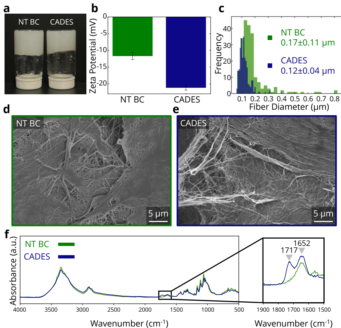
Fig. 1 Colloidal and chemical effects of DES treatment on bacterial cellulose. (a), Non-treated and CADES BC dispersions. (b), Zeta potential of non-treated and CADES BC. (c), Comparison of fiber diameters of non-treated and CADES BC. SEM of non-treated BC (d) and CADES BC (e) films. (f), FTIR spectra of non-treated and CADES BC films.
