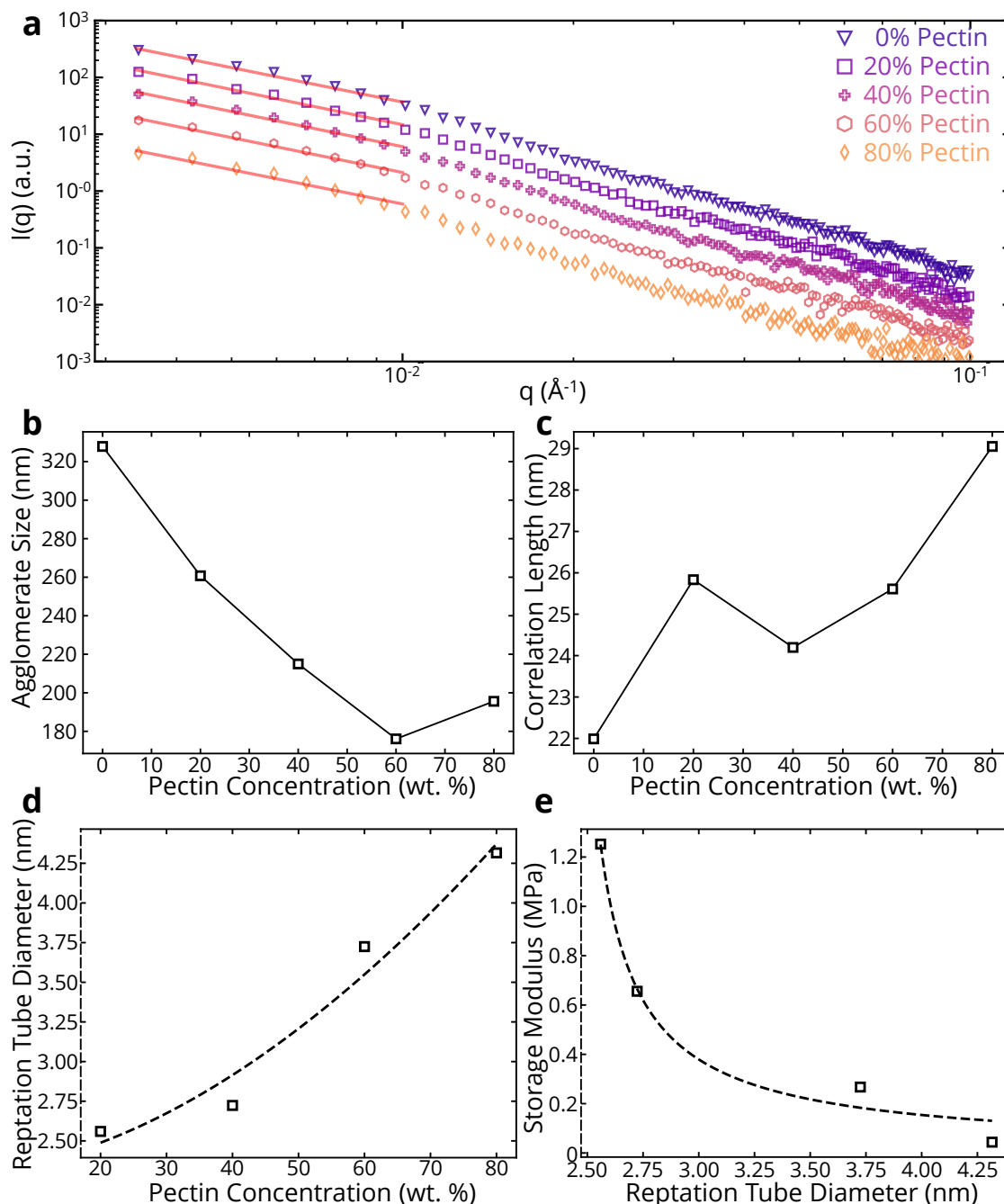
Fig. 4 Effects of Adding Pectin on Network Properties via SAXS. (a), SAXS data for CADES BC/pectin composites with a power-law fit in the low- q region. (b), Agglomerate size, (c), correlation length, (d), and reptation tube diameter of CADES BC/pectin composites. (e), Effect of reptation tube diameter on storage modulus of the colloids.
