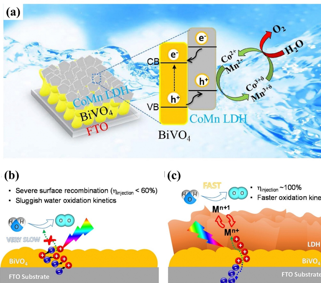
Fig. 7 (a) Schematic representation of PEC water splitting utilizing the \text{BiVO}_4/\text{CoMn-LDH} photoanode. Reproduced with permission from ref. 140, Copyright 2020, Elsevier; (b) and (c) Illustrative depiction of charge carrier dynamics during water oxidation on \text{BiVO}_4 and \text{BiVO}_4/\text{CoMn-LDH} photoelectrode. Reproduced with permission from ref. 141, Copyright 2019 Elsevier.
