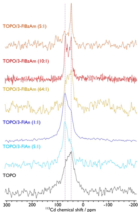
Fig. 4 ^{113}\text{Cd} MAS NMR spectra of CdS NCs with ligands indicated. A MAS frequency of 8 kHz was used for TOPO, 10 kHz was used for TOPO/3-FIAAn (1:1), and 12 kHz was used for TOPO/3-FIAAn (5:1), TOPO/3-FIBzAm (64:1), TOPO/3-FIBzAm (10:1), and TOPO/3-FIBzAm (5:1) CdS NCs. Vertical dashed lines highlight peak positions for wurtzite ( \sim 48 ppm) and sphalerite ( \sim 71 ppm) CdS NCs. See the ESI† for corresponding spectral fittings. Ratio of TOPO : fluorinated amine are by mass, as in Table 1.
