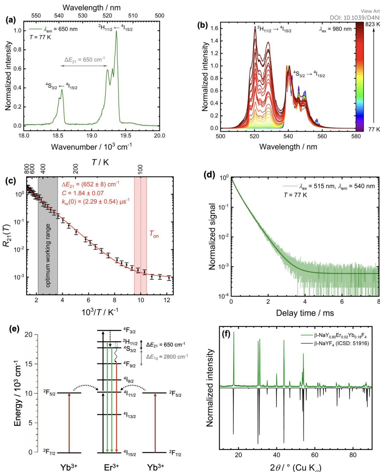
Figure 1. Characteristics of microcrystalline \beta -NaYF 4 : 2 mol% Er 3+ , 18 mol% Yb 3+ for luminescence Boltzmann thermometry. (a) High-resolution photoluminescence excitation spectra at T = 77 K (plotted against wavenumbers) upon monitoring the red ^4F_{9/2} \rightarrow ^4I_{15/2} -based emission at \lambda_{em} = 650 nm. The effective energy gap between the ^4S_{3/2} and ^2H_{11/2} level is indicated. (b) Temperature-dependent upconversion spectra of \beta -NaYF 4 : 2 mol% Er 3+ , 18 mol% Yb 3+ upon near infrared excitation ( \lambda_{ex} = 980 nm) between 77 K and 823 K. The spectra were normalized with respect to the emission peak at 540 nm. (c) Plot of the LIR of the two green emission bands of Er 3+ against reciprocal temperature in the measured temperature range. Integration ranges were between 510 nm and 533 nm as well as 533 nm and 555 nm, respectively. The red line corresponds to a fit according to eq. (x). Both the estimated onset temperature T_{on} and the optimum working range according to eq. (2) are indicated. (d) Luminescence decay curve of the ^4S_{3/2} \rightarrow ^4I_{15/2} -based emission ( \lambda_{em} = 540 nm, spectral bandwidth \Delta\lambda = 1.5 nm) upon direct excitation into the ^2H_{11/2} level ( \lambda_{ex} = 515 nm) at T = 77 K. The solid line represents an effective triexponential fit and gives an intensity-weighted average decay time of \langle\tau\rangle = 0.41 ms. (e) Schematic energy level scheme for the cooperative upconversion process between Yb 3+ and Er 3+ . Solid, straight arrows depict absorption (upward) or emission (downward) pathways. Relevant nonradiative processes in this work are indicated by curly black arrows. (f) Powder X-ray diffraction pattern (Cu K \alpha radiation) of as-synthesized microcrystalline \beta -NaYF 4 : 2 mol% Er 3+ , 18 mol% Yb 3+ compared to a diffraction pattern derived from single-crystal structure data of \beta -NaYF 4 (ICSD: 51916).
