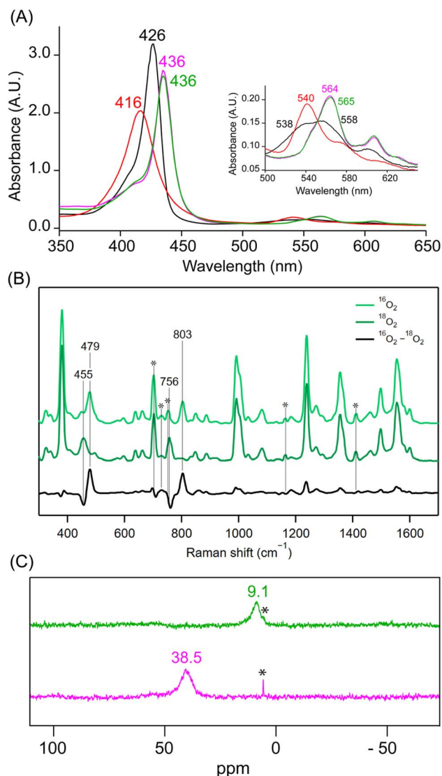
Fig. 2 (A) UV-vis spectra (in 9 : 1 DCM : THF at -40^{\circ}\text{C} ) for 50 \mu\text{M} solutions of [(THF) 2 (TPP)Fe III ] (black), [(THF)(TPP)Fe III (O 2 2- )] (red), [(THF)(TPP)Fe III (O 2 2- )] (pink), and [(4-Melm)(TPP)Fe III (O 2 2- )] (green). Inset shows the expanded Q-band region. (B) Resonance Raman spectra ( \lambda_{\text{ex}} = 457\text{ nm} ) collected for a 2 mM 9 : 1 DCM : THF frozen solution sample of [(4-Melm)(TPP)Fe III (O 2 2- )] - prepared with 16 O 2(g) (light green) and 18 O 2(g) (dark green); the difference spectrum is shown in black. (C) 2 H NMR spectra (in 9 : 1 DCM : THF at -40^{\circ}\text{C} ) for [(THF)(TPP-d 8 )Fe III (O 2 2- )] - (pink), and [(4-Melm)(TPP-d 8 )Fe III (O 2 2- )] - (green); *peaks correspond to the solvent.
