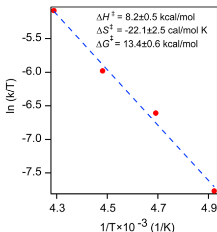
Fig. 5 Eyring analysis data showing the dependence of \ln(k/T) on 1/T for the reaction between a 50\ \mu\text{M} solution of [(ArO^-)(TPP)Fe^{III}(O_2^{2-})]^{2-} and acetophenone oxime at -40 , -50 , -60 and -70^\circ\text{C} . Solvent = 9 : 1 DCM : THF.
