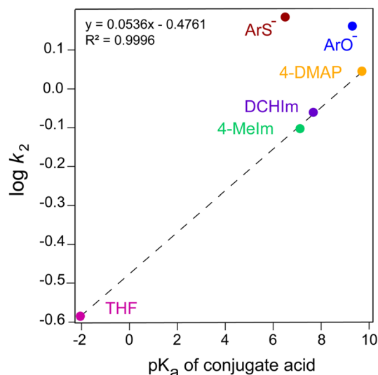
Fig. 4 The correlation between \log k_2 values for [(B)(TPP)Fe^{III}(O_2^{2-})]^- mediated acetophenone oxime oxidation reactions (in 9 : 1 DCM : THF at -40^\circ\text{C} ) and the pK_a values of conjugate acids of the axially ligating B ligands, where B = THF (magenta), 4-Melm (green), DCHIm (purple), 4-DMAP (orange), ArO^- (blue) and ArS^- (brick red).
