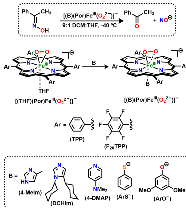
Scheme 1 Generalized oxime oxidation reaction scheme facilitated by heme peroxy intermediates and the divergent exogenously added axial ligands evaluated in this study.
