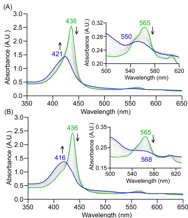
Fig. 3 (A) Electronic absorption spectral changes observed (in 9 : 1 DCM : THF at -40^{\circ}\text{C} ) during the reaction of a 50 \mu\text{M} solution of (A) [(4-Melm)(TPP)Fe III (O 2 2- )] - and (B) [(4-DMAP)(TPP)Fe III (O 2 2- )] - with 200 equiv. of acetophenone oxime (green: initial six coordinate heme-PO complex; blue: final ferric product). Insets show the expanded Q-band regions, and arrows indicate the direction of peak transition.
