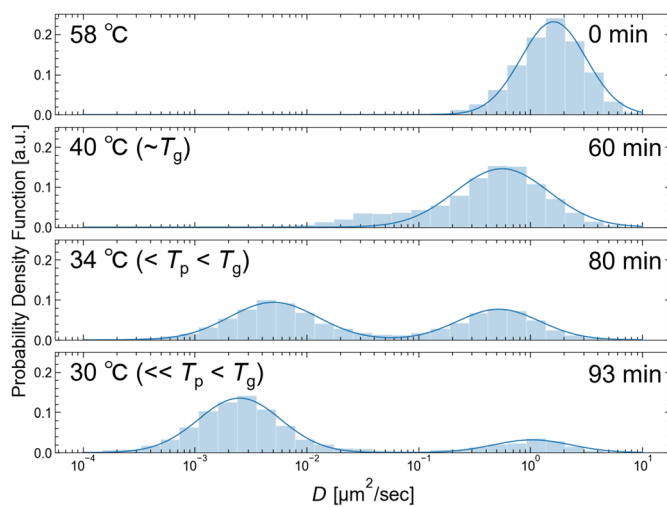
Fig. 5 Histogram of time-averaged D obtained from MSD with \tau \sim 1 s. The temperature was regulated upon (a) a slow quenching from 80 to 25 °C ( < T_p = 35 °C) with 0.3 °C \text{min}^{-1} or (b) maintained to be 40 °C ( \sim T_g ). The number of data points is (a) 33 000–64 000 and (b) approximately 40 000, respectively. The solid line in (a) and (b) is a fitting line with a double Gaussian and a single Gaussian, respectively.
