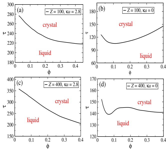
Fig. 5 Transition lines delimiting the onset of sheet layering across the transversal direction, considering both screened and unscreened dipoles, and two representative charges of Z = 100q (top graphs) and Z = 400q (lower graphs).
