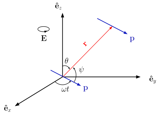
Fig. 1 Sketch of the geometry of point dipoles oscillating at angular frequency \omega along a circle of radius p lying at the xy plane, and separated by a distance r .
