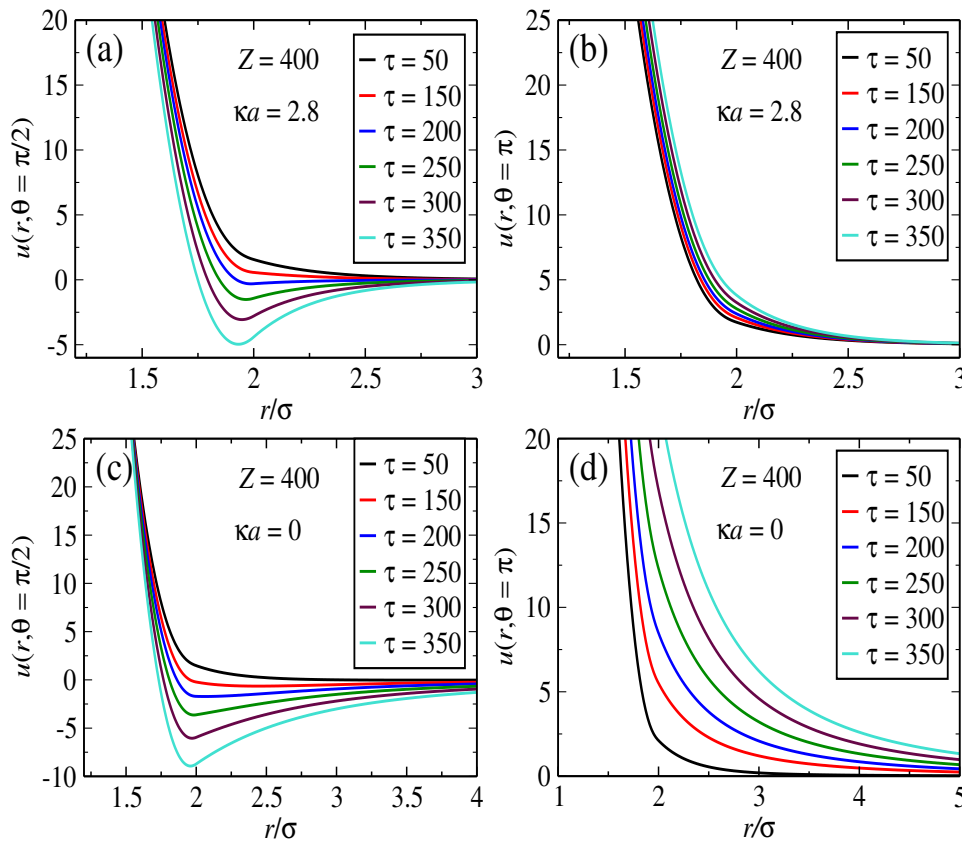
Fig. 2 Effective potential between ionic microgels induced by a CP field, at different dipole strengths. Top panels correspond to fully screened dipole interactions ( \kappa_l = \kappa ), whereas at the bottom curves results for unscreened interactions ( \kappa = 0 ) are shown. In all cases, the monopole charge is made of Z = 400 elementary charges.
