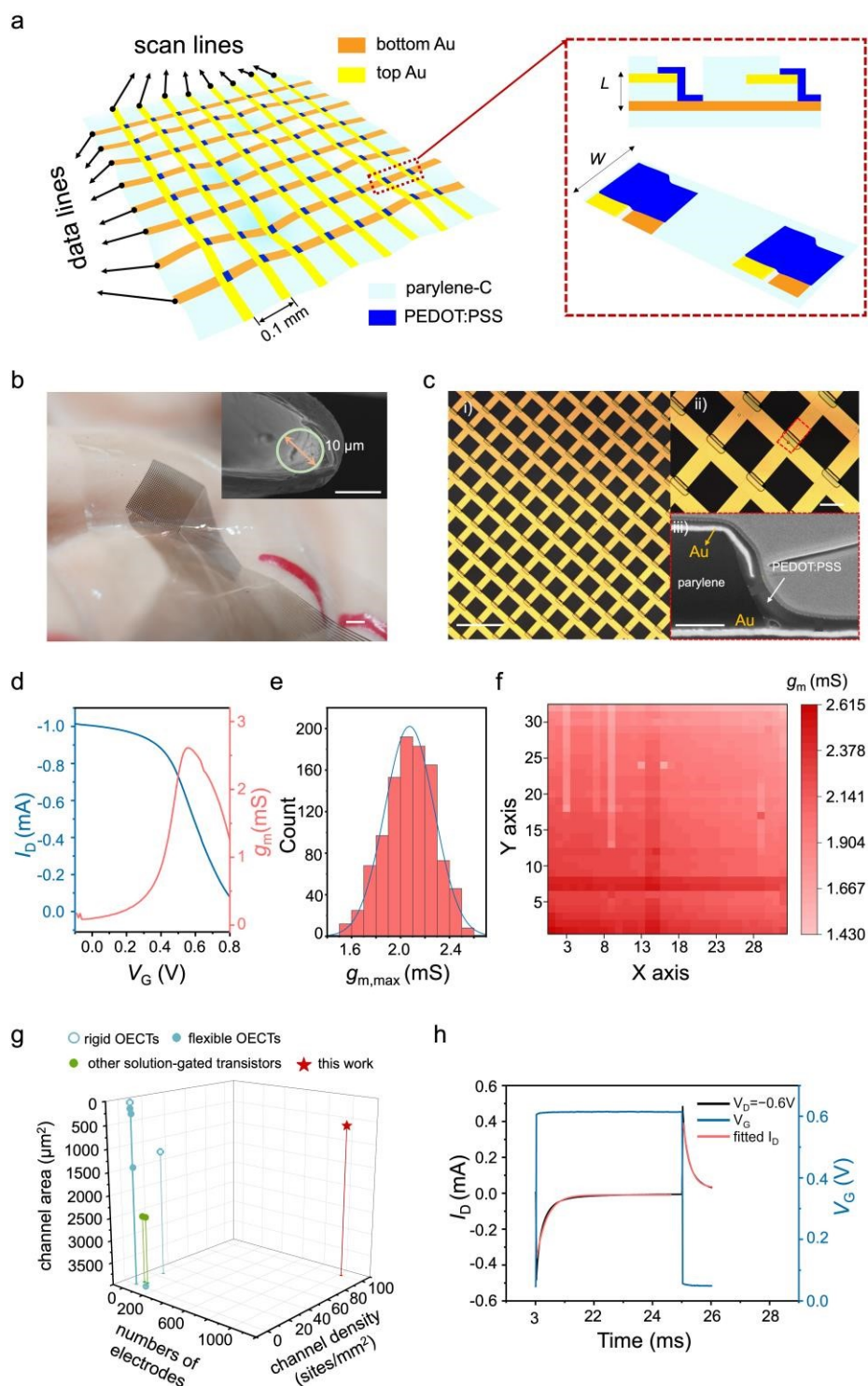
Figure 1. Design and the performance of the ultraflexible, high-density vOECT array. a) Left panel: Illustration of the vOECT array on a flexible parylene substrate. Right panel: zoom-in schematics of two adjacent pixels, showing both the side view and the top view. b) A photograph showing the ultraflexible, high-density vOECT array attached to a brain model. Scale bar, 1 mm. Inset is a scanning electron microscopic (SEM) image of a 4.2 \mu\text{m} -thick vOECT bent to a 5 \mu\text{m} radius. Scale bar, 10 \mu\text{m} . c) Optical micrograph of an ultraflexible, 1,024-channel vOECT array with a density of 10,000 transistors \text{cm}^{-2} . Scale bar, 200 \mu\text{m} . The upper inset displays a magnified image of the vOECT array (ii). Scale bar, 50 \mu\text{m} .
