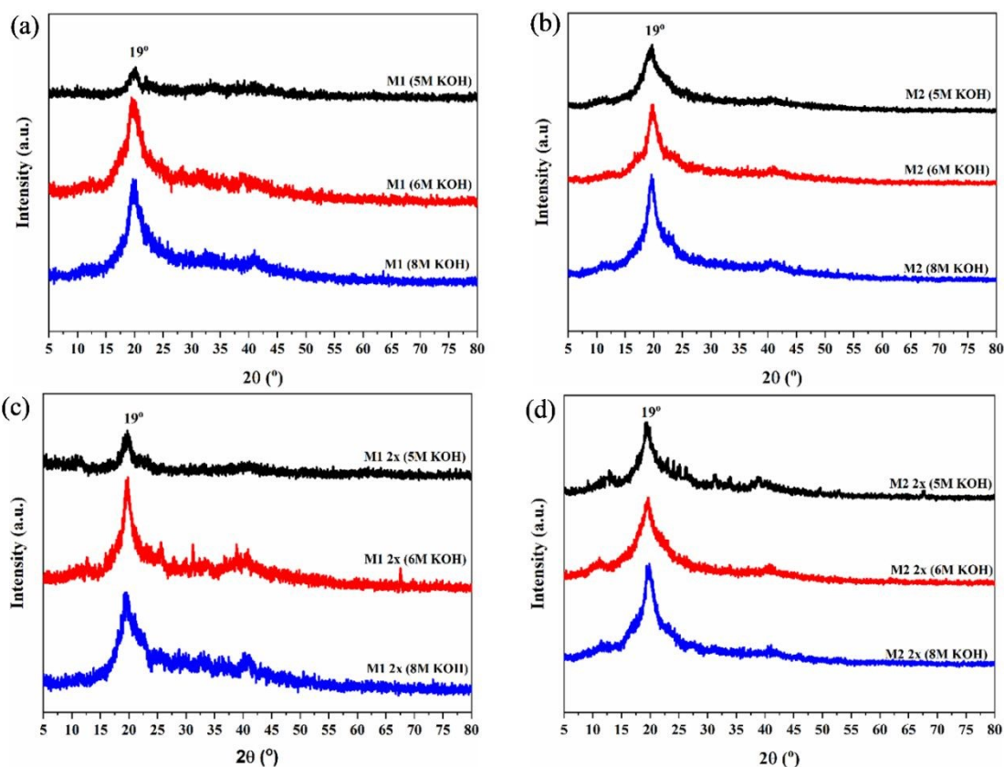
Figure 3. XRD patterns of (a) M1, (b) M2, (c) M1 2x and (d) M2 2x samples under different KOH concentrations for activations.
