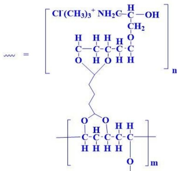
Figure 8. Hofmann elimination and S N 2 substitution mechanism in QPVA membranes.
