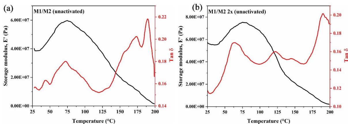
Figure 6. DMA curve (a) M1/M2 (unactivated) and (b) M1 2x/M2 2x (unactivated) QPVA membranes.
