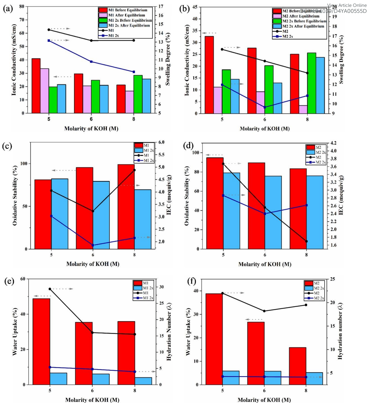
Figure 7. (a) Ionic conductivity and swelling degree for M1 and M1 2x membranes at different KOH molarities, (b) Ionic conductivity and swelling degree for M2 and M2 2x membranes at different KOH molarities, (c) Oxidative stability and IEC values for M1 and M1 2x membranes at different KOH molarities. (d) Oxidative stability and IEC values for M2 and M2 2x membranes at different KOH molarities. (e) Water uptake and hydration number for M1 and M1 2x membranes at different KOH molarities. (f) Water uptake and hydration number for M2 and M2 2x membranes at different KOH molarities.
