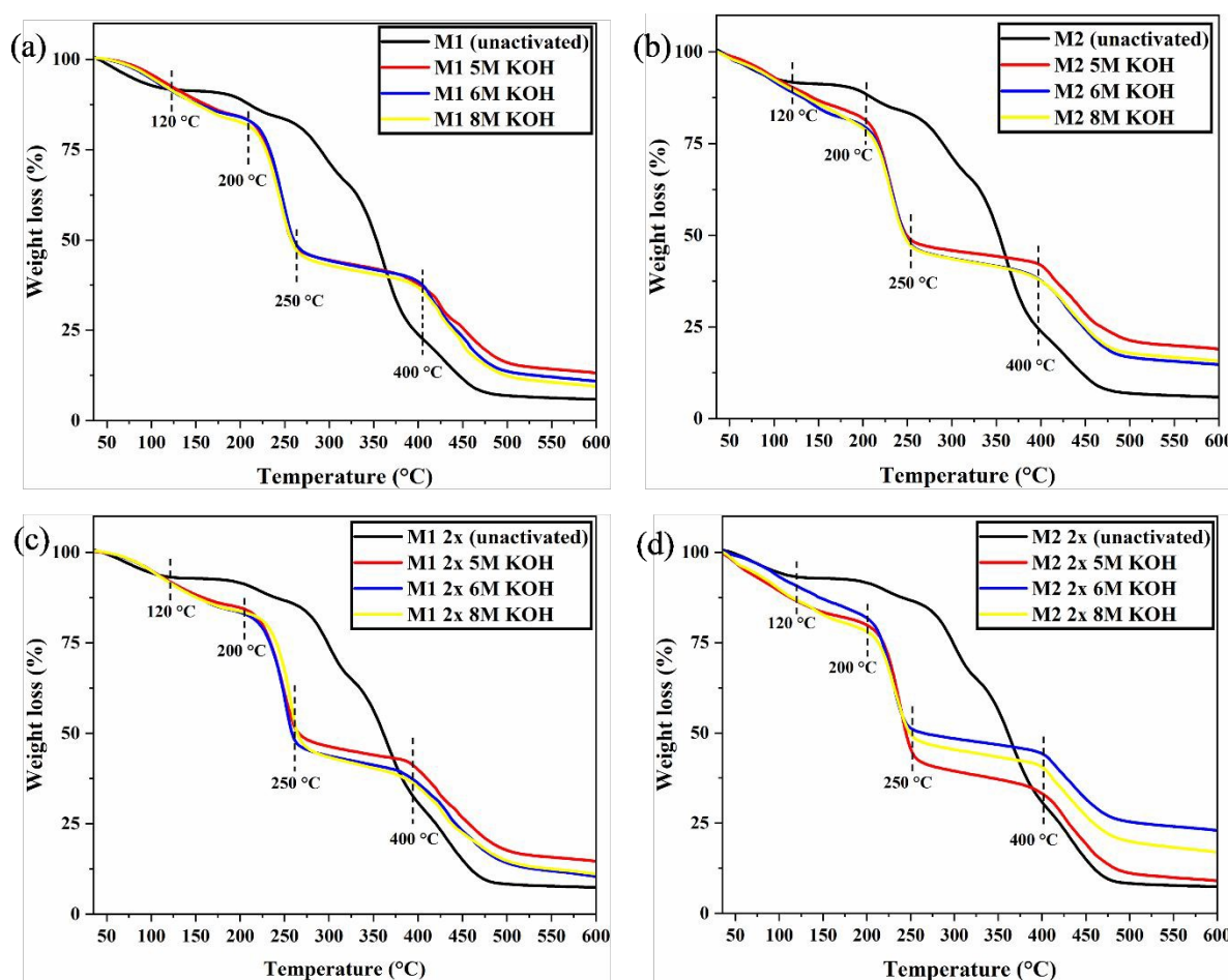
Figure 5. TGA curves of (a) M1, (b) M2, (c) M1 2x and (d) M2 2x for comparison of unactivated and different KOH concentration of activation.
