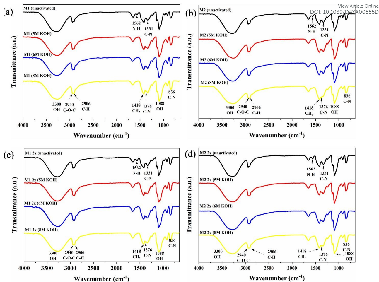
Figure 2. FT-IR spectra of QPVA membranes (a) M1, (b) M2, (c) M1 2x and (d) M2 2x samples.
