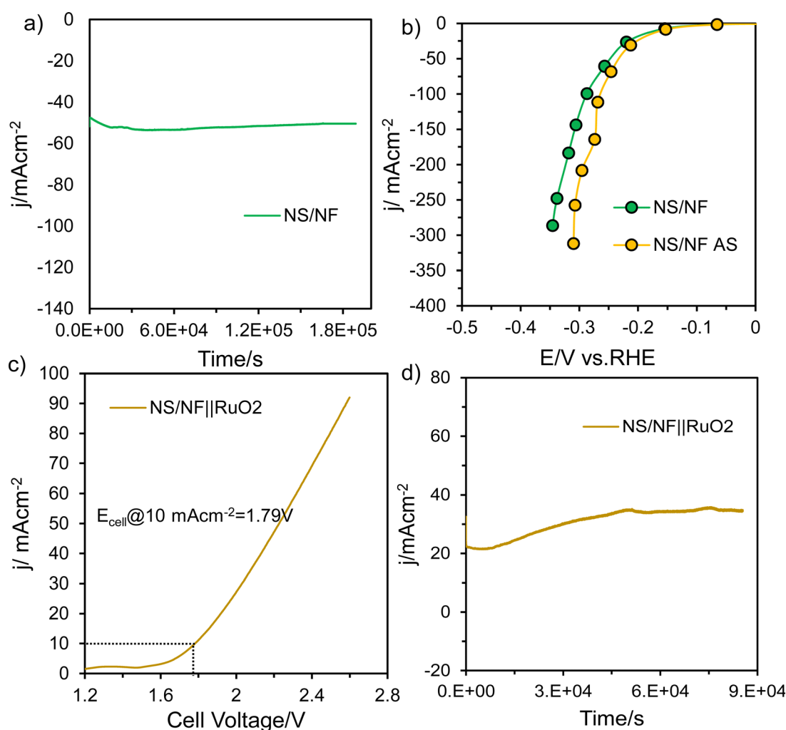
Fig. 5 (a) i - t curve demonstrating the durability of NS/NF catalyst for HER at a constant potential in 1.0 M KOH, (b) SCV curves of NS/NF before and after HER stability, (c) polarisation curves showing overall cell voltage and (d) chronopotentiometry curves for NS/NF||RuO 2 in 1.0 M KOH.
