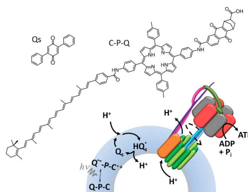
Fig. 15 An artificial photosynthetic vesicle. 36
