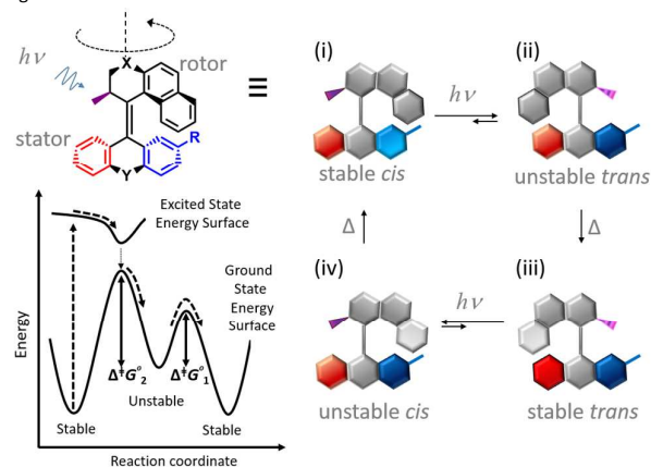
Fig. 8 Light-driven unidirectional intramolecular rotation of a synthetic molecular motor. 9
