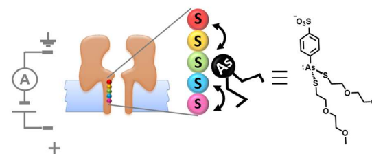
Fig. 18 Stochastic walking of a small molecule within a transmembrane nanopore. 40
