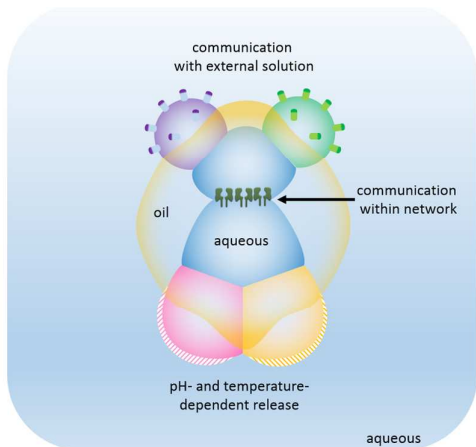
Fig. 25 Droplet multisomes that operate in aqueous environments. 49
