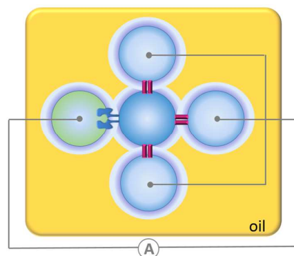
Fig. 24 A simple circuit constructed from a droplet interface bilayer network connected by an \alpha -haemolysin pore and bacteriorhodopsin. 48
