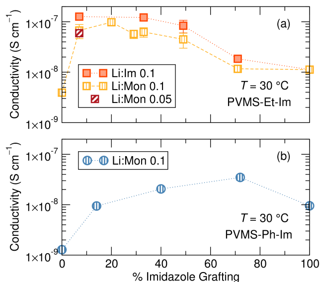
Figure 4: Total ionic conductivity for the (a) ethane-imidazole and (b) phenyl-imidazole series as a function of the percentage of monomers containing an imidazole sidechain.
