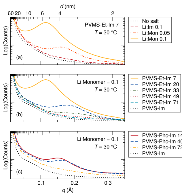
Figure 2: SAXS shows change in aggregation peak location and intensity with (a) salt concentration in the ethane-imidazole polymer containing 7% imidazole, and with imidazole grafting density at a constant \text{Li}^+ to monomer molar ratio of 0.1 for the (b) ethane-imidazole and (c) phenyl-imidazole polymer series. Polymer without imidazole present is not shown here due to poor solubility of the salt and shifting of ion aggregation peak
