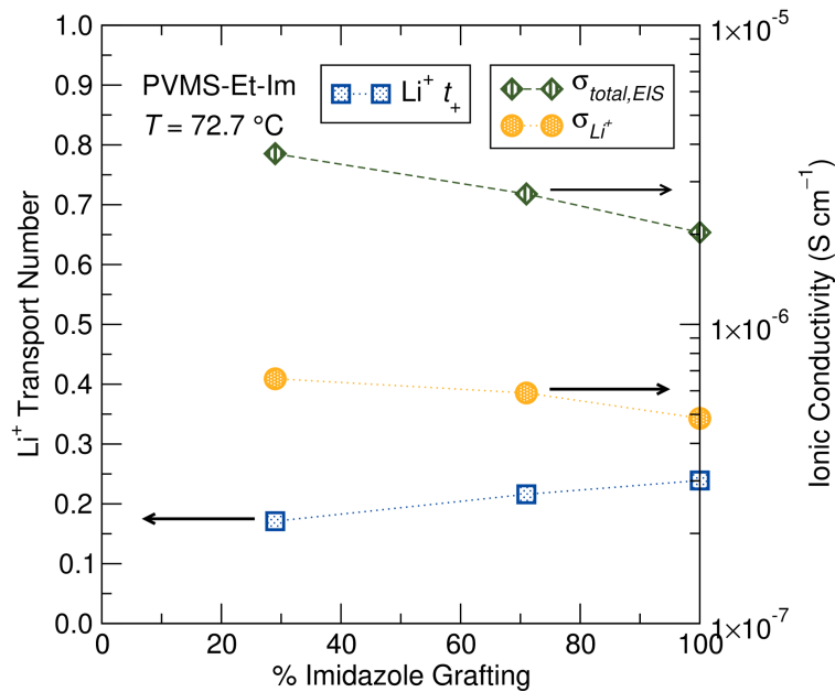
Figure 6: Transport numbers ( \text{Li}^+ t_+ ), total EIS-measured ionic conductivity ( \sigma_{\text{total,EIS}} and adjusted \text{Li}^+ -ion conductivity ( \sigma_{\text{Li}^+} ) for the three PVMS-Et-Im grafting density polymers measured using PFG-NMR at 72.7 °C. All samples consist of a 0.1 Li:monomer ratio of LiTFSI added to the polymer.
