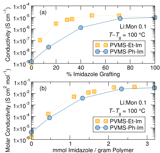
Figure 5: (a) T_g -normalized total ion conductivity versus grafting density for the ethane-imidazole and phenyl-imidazole polymer series at a \text{Li}^+ :monomer ratio of 0.1. (b) The T_g -normalized conductivity can be approximately normalized by salt concentration (to obtain molar conductivity) and plotted against the mmol of imidazole per gram polymer which acts as a proxy for imidazole molar volume. These data now show a very similar trend between the ethane and phenyl series. Error bars are smaller than symbols.
