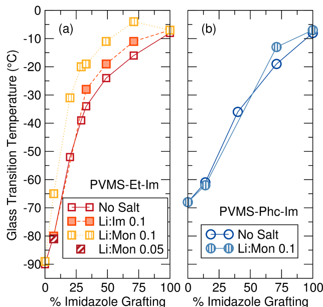
Figure 3: Polymer glass transition temperature ( T_g ) versus grafting density for the (a) ethane-imidazole and (b) phenyl-imidazole polymer grafting series. A lower imidazole content results in lower T_g due to the removal of the polar and hydrogen-bonding groups. The lower steric bulk of the ethane side chain results in a lower T_g ( -90 °C) than the fully phenyl-functionalized polymer ( -68 °C).
