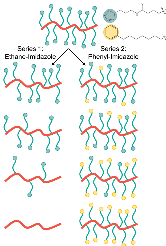
Figure 1: Schematic representation of the polymer series synthesized for this study. Series 1 changes the imidazole grafting density by replacing imidazole with a non-bulky ethane inert side chain, while Series 2 replaces the imidazole with a phenyl inert side chain to maintain similar steric bulk.
