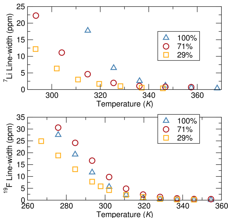
Figure 7: (a) ^7\text{Li} NMR and (b) ^{19}\text{F} NMR peak width, as a function of temperature. All samples consist of a 0.1 Li:monomer ratio of LiTFSI added to the polymer.
