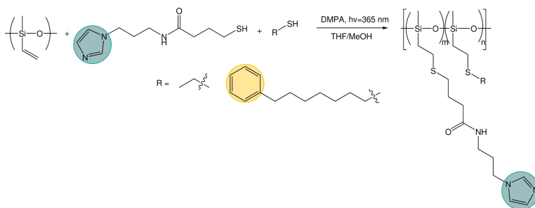
Scheme 1: Synthesis of the polymer grafting series was achieved using thiol-ene click chemistry to attach various ratios of imidazole thiol and either ethane thiol or phenyl thiol to a poly(vinyl methyl siloxane) backbone.
