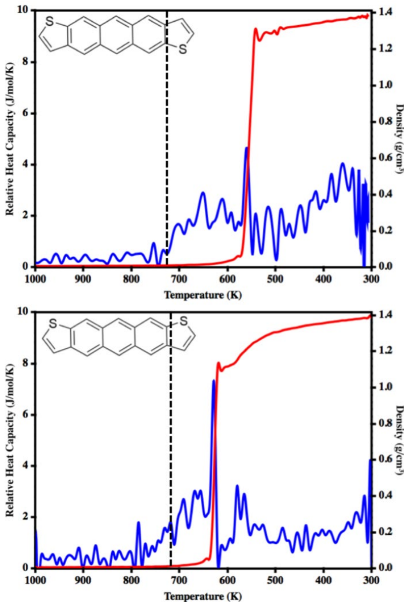
Figure 3. Relative heat capacity (blue) and simulation box density (red) of anti ADT (top) and syn ADT (bottom) as the system is cooled from 1000 K to 300 K. The experimental melting points of the anti ADT (725 K) and syn ADT (720 K) are highlighted with dashed, black lines.
