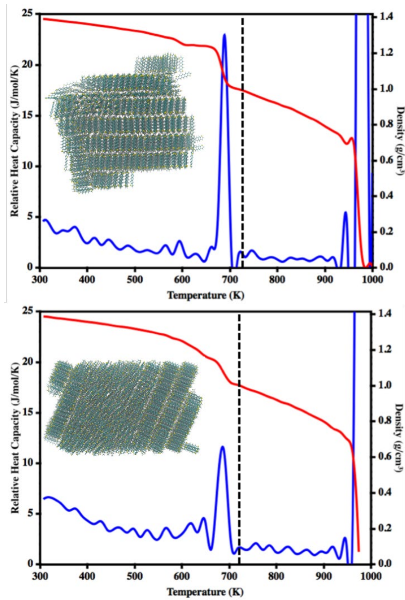
Figure 9. Relative heat capacity (blue) and simulation box density (red) of antiADT (top) and synADT (bottom) as the recrystallized system is heated from 300 K to 1000 K. The experimental melting points of the antiADT (725 K) and synADT (720 K) are highlighted with dashed, black lines. The insets show the respective initial system morphologies prior to reheating.
