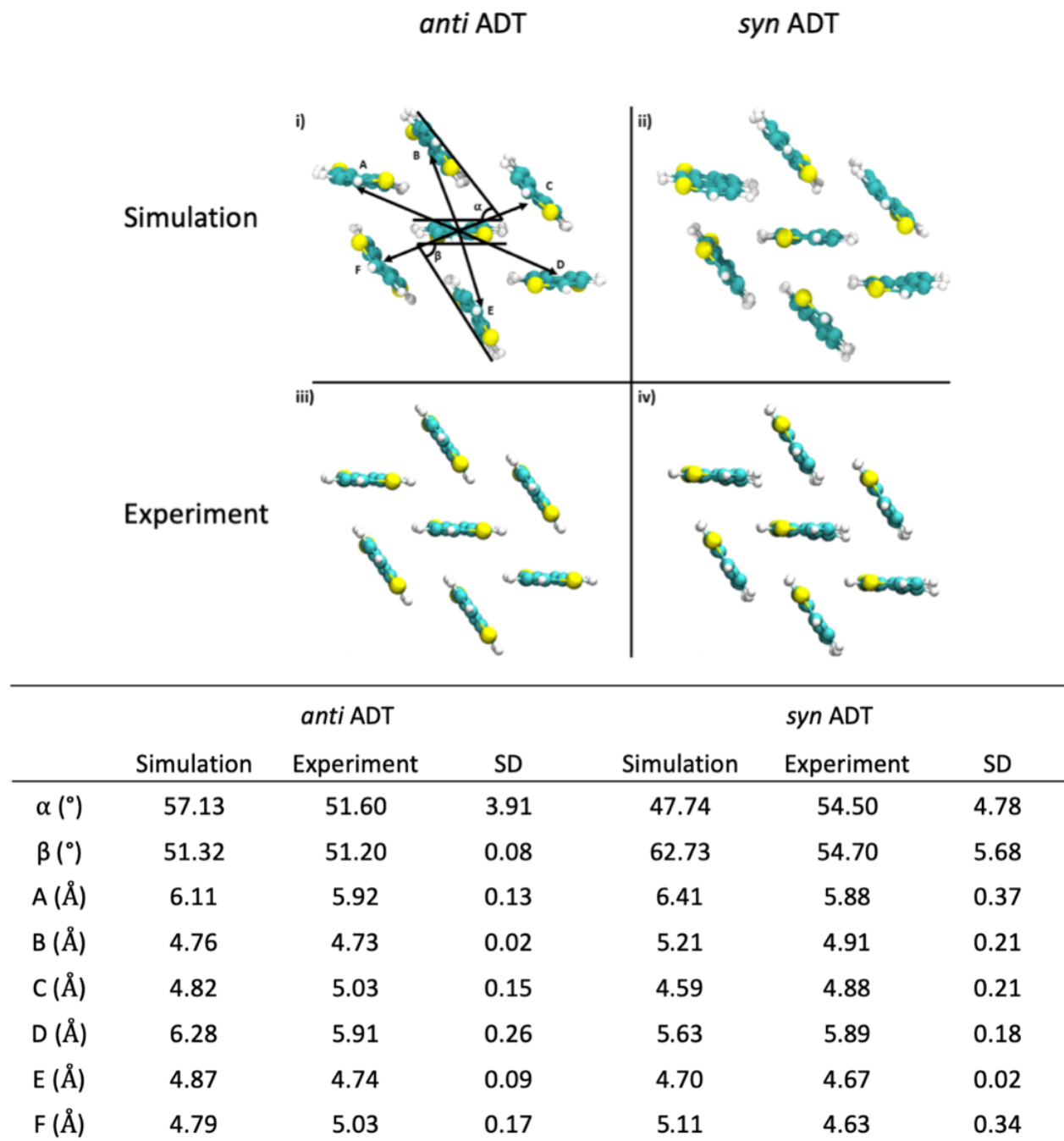
Figure 8. Comparison of crystalline packing of anti ADT and syn ADT as extracted from a series of snapshots after simulation box crystallization to the experimentally reported crystal structure. Molecular distances and angles are reported in table with standard deviations for each angle and distance.
