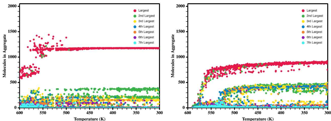
Figure 5. Number of molecules in each crystalline aggregate in antiADT (left) and synADT (right) as the simulation boxes are cooled. Note a total of 1600 antiADT molecules and 2000 synADT molecules.
