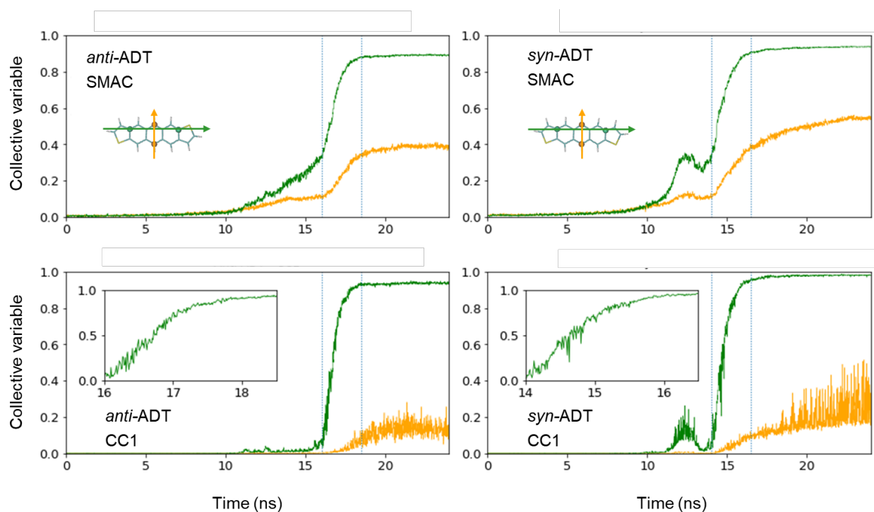
Figure 6. Normalized crystallinity descriptor collective variables (CV) SMAC (top row) and CC1 (bottom row) derived for the cooling of antiADT and synADT as a function of simulation time in terms of the long-axis (green) and short-axis (yellow) vectors. The inserts in the figures in the bottom row highlight the CV changes during crystallization, which fall between the dotted lines in the full images.
