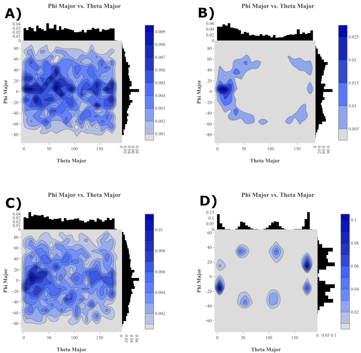
Figure 7. Relative molecular long-axis alignment for antiADT (A, B) and synADT (C, D) upon initial system condensation (A, C) and the final crystallized system (B, D). Theta is the angle between the long axes of two molecules while phi is their relative rotation with respect to each other.
