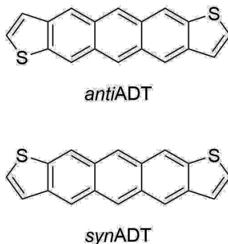
Figure 1. Chemical structures of the anti - ( anti ADT) and syn - ( syn ADT) forms of anthradithiophenes (ADT).
