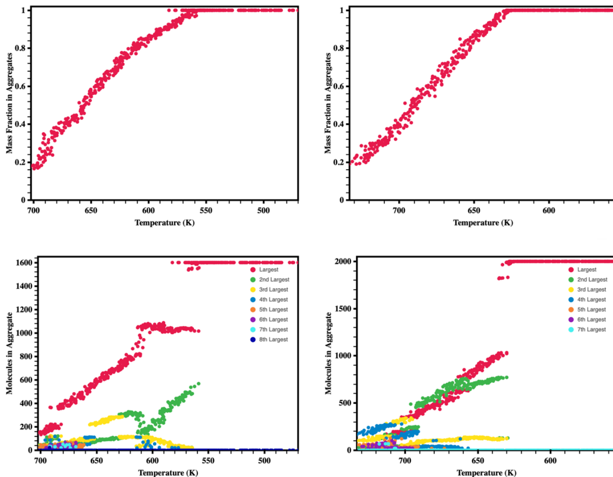
Figure 4. (Top) Fraction of total simulation mass present within aggregates versus free molecules for antiADT (left) and synADT (right). (Bottom) Total number of molecules within the largest aggregates present within the simulation boxes prior to aggregates coalescing. Note differing X-axis scales for antiADT and synADT due to aggregate formation initiating at different temperatures (Figure 1).
