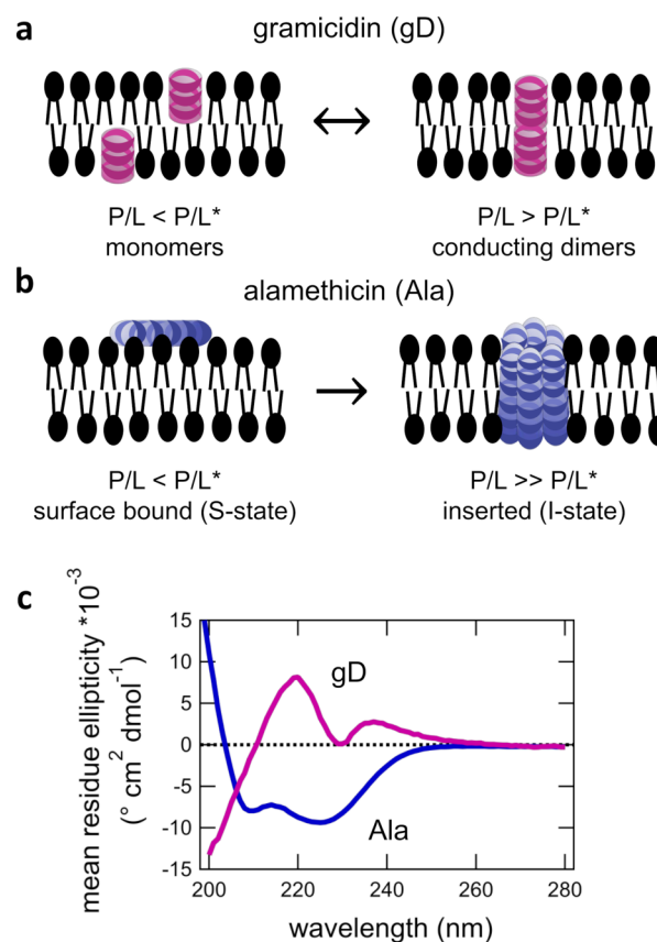
Fig. 1 Cartoon illustration of transmembrane channel formation by (a) gD and (b) Ala. Corresponding circular dichroism (CD) data showing the \beta^{6.3} -helical and \alpha -helical structures for gD and Ala in DMPC lipid membranes at 35^{\circ}\text{C} \pm 2^{\circ}\text{C} at a peptide to lipid ratio ( P/L ) of 1/130 and 1/150, respectively.
