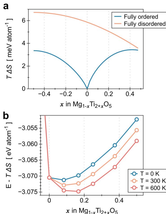
Figure 7. (a) Contribution of mixing entropy at 300 K for \text{Mg}_{1-x}\text{Ti}_{2+x}\text{O}_5 , ranging from the fully ordered experimental structure (all Mg/Ti fill the M1/M2 sites, respectively) to fully disordered (random occupation of M1/M2 states). Note that the mixing entropy for the fully ordered \text{MgTi}_2\text{O}_5 ( x = 0 ) is 0. (b) Formation free energy of \text{Mg}_{1-x}\text{Ti}_{2+x}\text{O}_5 at zero temperature, room temperature, and elevated temperature; the entropic stability is observed to be significant.
