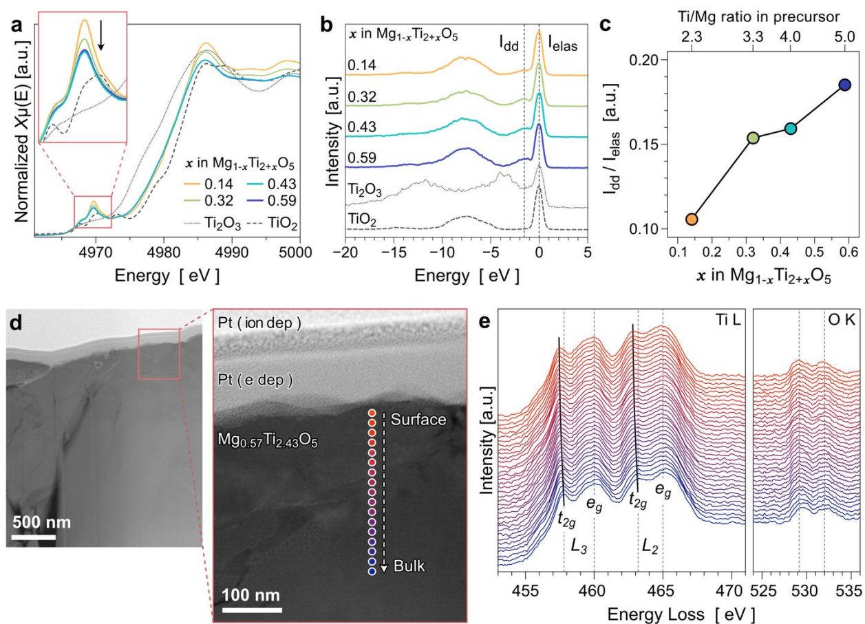
Figure 5. Chemical analysis of synthesized MTOs ( x = 0.14, 0.32, 0.43, and 0.59 in \text{Mg}_{1-x}\text{Ti}_{2+x}\text{O}_5 ). (a) Ti K-edge XANES results. The inset presents an enlarged view of the pre-edge region. (b) RIXS spectra collected with the excitation energy of 458 eV. Standard spectra of \text{Ti}^{3+} ( \text{Ti}_2\text{O}_3 ) and \text{Ti}^{4+} ( \text{TiO}_2 ) are included as references. (c) Relative peak areas of I_{\text{dd}}/I_{\text{elas}} plotted as a function of x .
