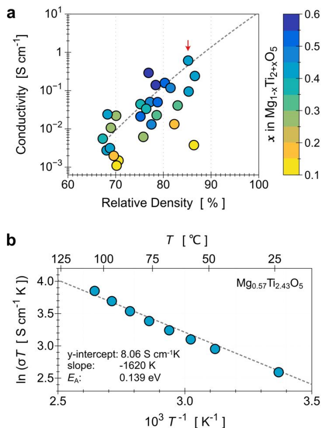
Figure 4. (a) Relation between the electrical conductivity, relative density of the MTO pellet, and relative Ti content ( x in \text{Mg}_{1-x}\text{Ti}_{2+x}\text{O}_5 ). Note that the dotted line is the fit of the MTOs with a similar valence state of Ti ( 3.65 \pm 5\% ), which is the condition that resulted in the best conductivity in the present study ( 6.09 \times 10^{-1} S cm at \text{Mg}_{0.57}\text{Ti}_{2.43}\text{O}_5 , indicated by the red arrow). (b) Temperature dependence of the conductivity of \text{Mg}_{0.57}\text{Ti}_{2.43}\text{O}_5 , plotted as \ln(\sigma T) vs. T^{-1} . The dotted line is the best-fit line with Eq. (1).
