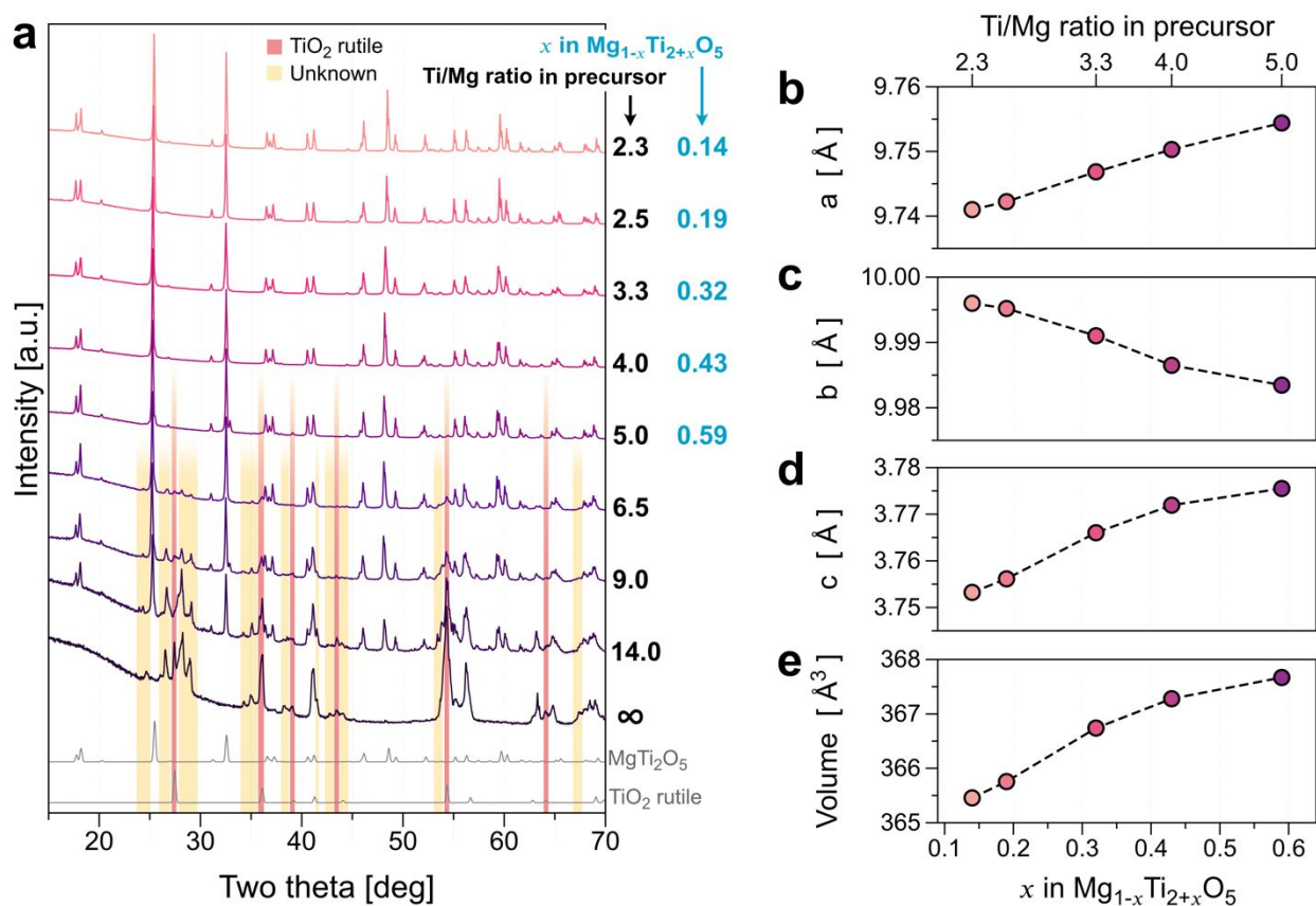
Figure 3. Series of XRD results of MTO synthesized from precursor with a \text{TiO}_2 content greater than \text{Ti/Mg} = 2.3 . Note that the remaining \text{TiO}_2 rutile phase (indicated by the red box) appears in MTOs ( \text{Ti/Mg} > 4.0 ) from the excessive Ti in the precursor. (b-e) Relations between the unit-cell parameters and volume as a function of x in \text{Mg}_{1-x}\text{Ti}_{2+x}\text{O}_5 .
