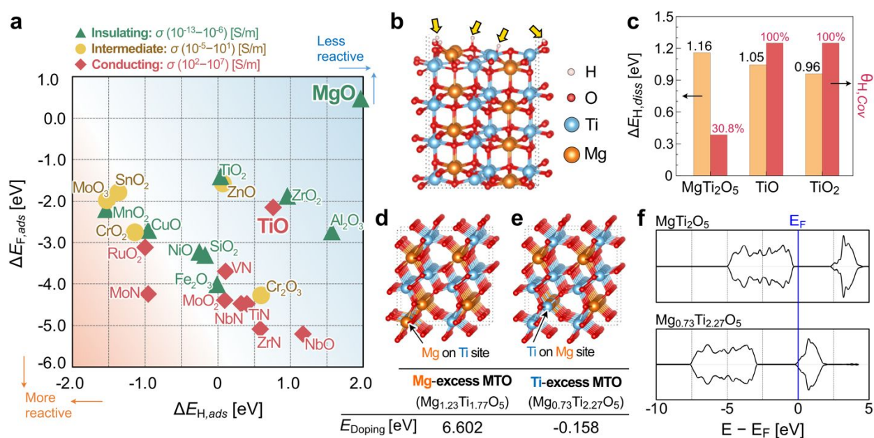
Figure 1. (a) Correlation observed between \Delta E_{\text{H,ads}} and \Delta E_{\text{F,ads}} after DFT single-adsorption calculations. (b) Hydrogen dissociation on a (110) \text{MgTi}_2\text{O}_5 slab model and (c) comparison of the hydrogen dissociation energy ( \Delta E_{\text{H,diss}} ) and hydrogen coverage ratio ( \theta_{\text{H,Cov}} ) of each Ti oxide. Note that only a few oxygen sites ( \sim 30.8\% ) showed hydrogen adsorption (denoted by the yellow arrows), suggesting \text{MgTi}_2\text{O}_5 is more protective in an acidic environment. Illustration of (d) \text{Mg}_{1.23}\text{Ti}_{1.77}\text{O}_5 and (e) \text{Mg}_{0.73}\text{Ti}_{2.27}\text{O}_5 structures, where an excessive Mg or Ti atom is occupying the Ti or Mg site
