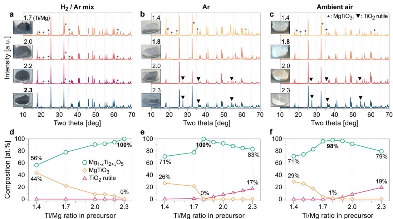
Figure 2. (a–c) XRD results and optical images of MTOs from various ratios of the precursor mixture and various gas environments. (d–f) Composition curves of the products as a function of the Ti/Mg molar ratio in the precursor mixture. Each column of the figure refers to the MTO series synthesized under (left) 2% \text{H}_2/\text{Ar} mixed gas, (center) Ar gas, and (right) ambient air environment. Note that the amount of the rutile phase (denoted as ▼) increases with increasing Ti content in the precursor, whereas the \text{MgTiO}_3 (denoted as *) content in the product increases with decreasing Ti content in the precursor.
