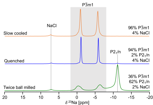
Fig. 2 23 Na ss-NMR spectra for twice ball milled (bottom), quenched (middle), and slow cooled (top) \text{Na}_2\text{ZrCl}_6 samples. Resonances assigned to the \text{P}\bar{3}m1 polymorph are within the grey box, while the prismatic Na site of the \text{P}2_1/n structure is on the dotted line to its right. For each sample, the molar % of Na in each phase is shown on the right hand side of the spectrum. Spectra were obtained at a 10 kHz spinning speed, resulting in a sample temperature of 52 °C.
