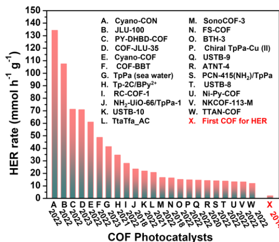
Fig. 7. Representative COF photocatalysts with exceptional H 2 evolution rates (>11 mmol g -1 h -1 ) using Pt or Cu (II) as co-catalyst under visible-light irradiation. Corresponding references are summarised in Table 3.
