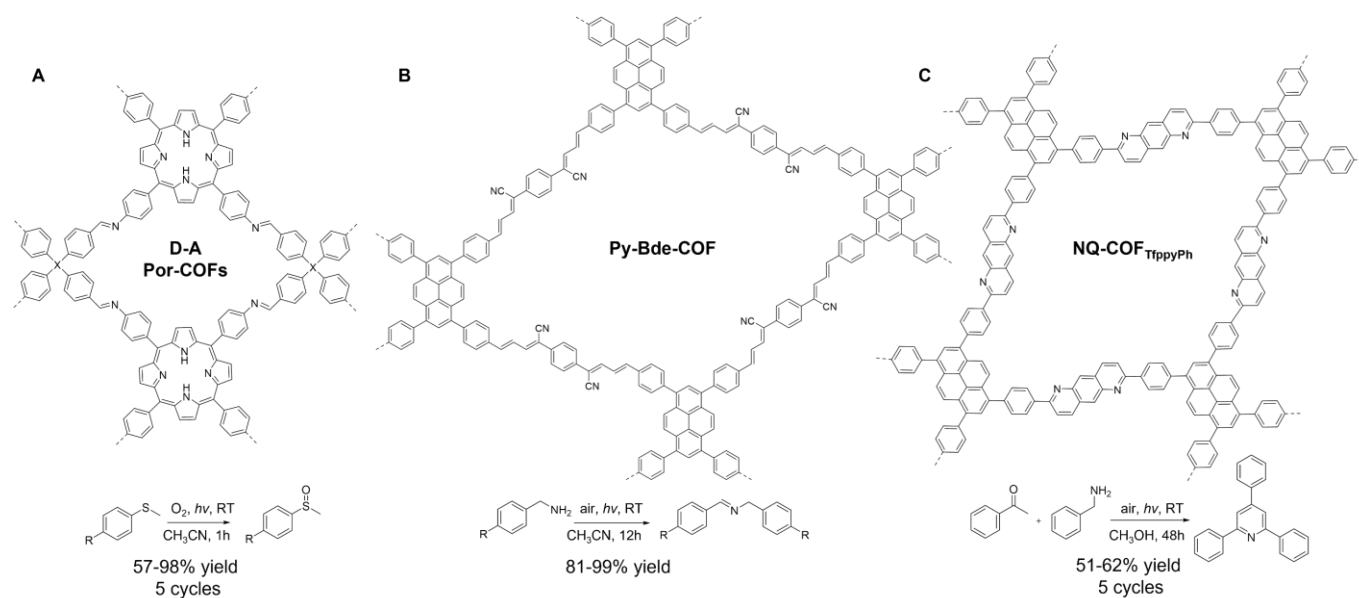
Fig. 6. Schematics of (A) D-A por-COFs, (B) buta-1,3-diene-linked Py-Bde-COF, and (C) NQ-COF for visible-light-driven photoredox catalysis.
