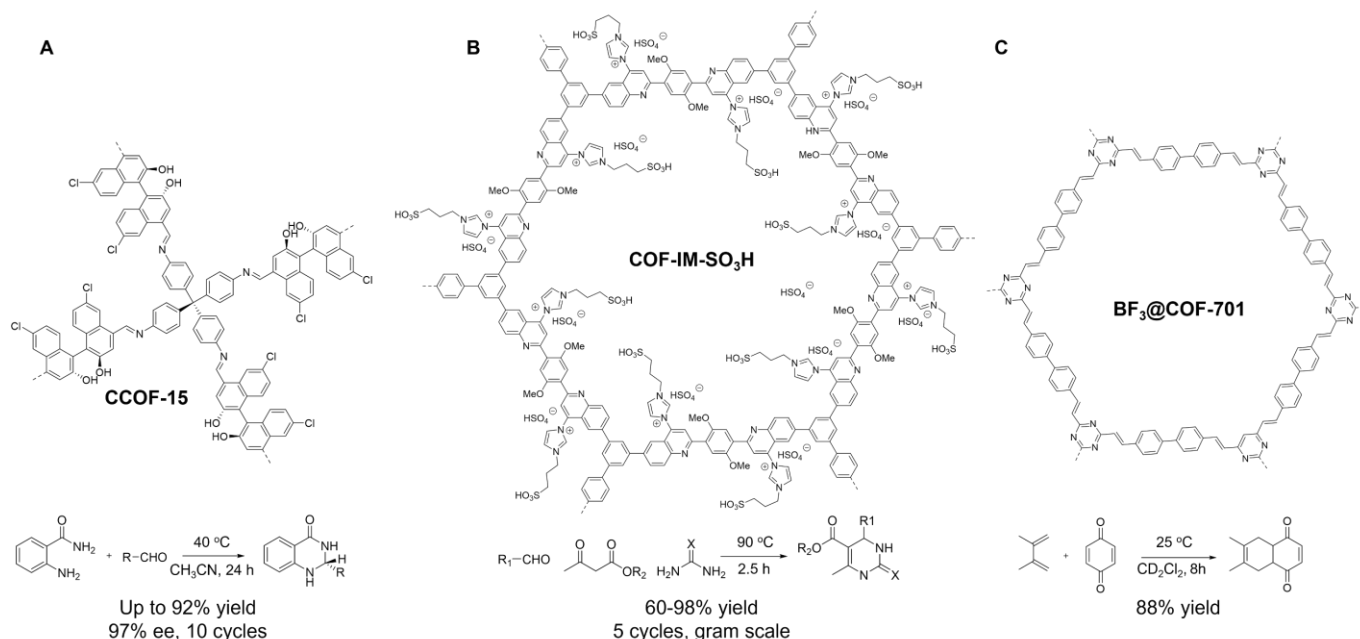
Fig. 2. Schematics of (A) 3D CCOF-15 with chiral acidic linkers, (B) COF-IM-SO 3 H made via PSM, (C) BF 3 /COF-701 as solid acids for thermocatalysis.
