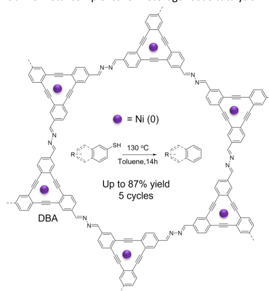
Fig. 4. Schematic of a Ni-Doped dehydrobenzoannulene (DBA)-containing COF for the reductive cleavage of aryl C-S bonds.
