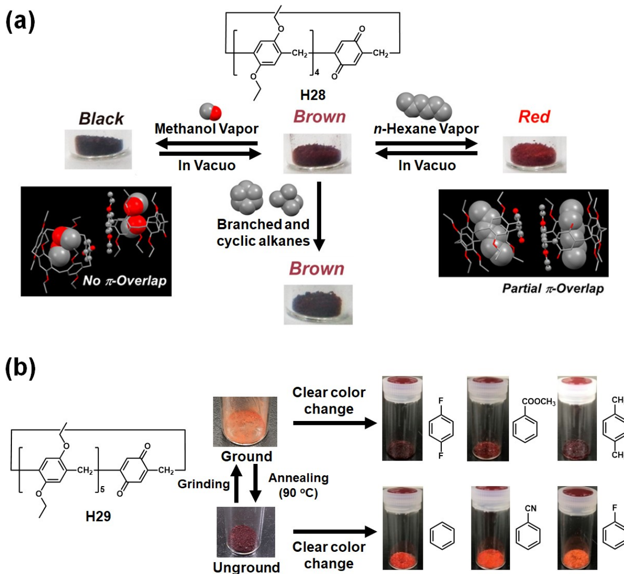
Figure 9. (a) Schematic representation of the vapochromism of H28 . Reproduced with permission from reference 141 (Copyright 2017 American Chemical Society). (b) Schematic representation of the vapochromism and mechanochromism of H29 . Reproduced with permission from reference 142 (Copyright 2020 Royal Society of Chemistry).
