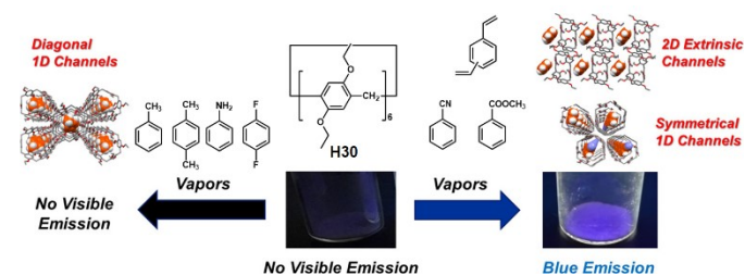
Figure 11. Schematic representation of the turn-on vapoluminescence of H30 in response to aromatic vapors. Reproduced with permission from reference 145 (Copyright 2020 American Chemical Society).
