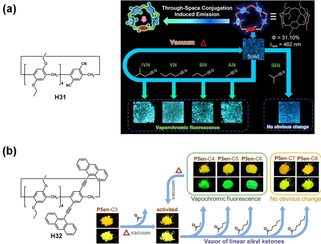
Figure 12. (a) Schematic representation of the vapoluminescence of H31 in response to common nitrile vapors. Reproduced with permission from reference 146 (Copyright 2022 American Chemical Society). (b) Schematic representation of the vapoluminescence of H32 in response to ketone vapors. Reproduced with permission from reference 147 (Copyright 2019 American Chemical Society).
