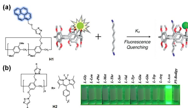
Figure 2. (a) Fluorescence quenching by photoinduced electron transfer between H1 and aliphatic amines. Reproduced with permission from reference 46 (Copyright 2011 American Chemical Society). (b) Fluorescence enhancement of H2 for selective detection of L-asparagine from amino acids. Reproduced with permission from reference 88 (Copyright 2020 Elsevier Inc).
