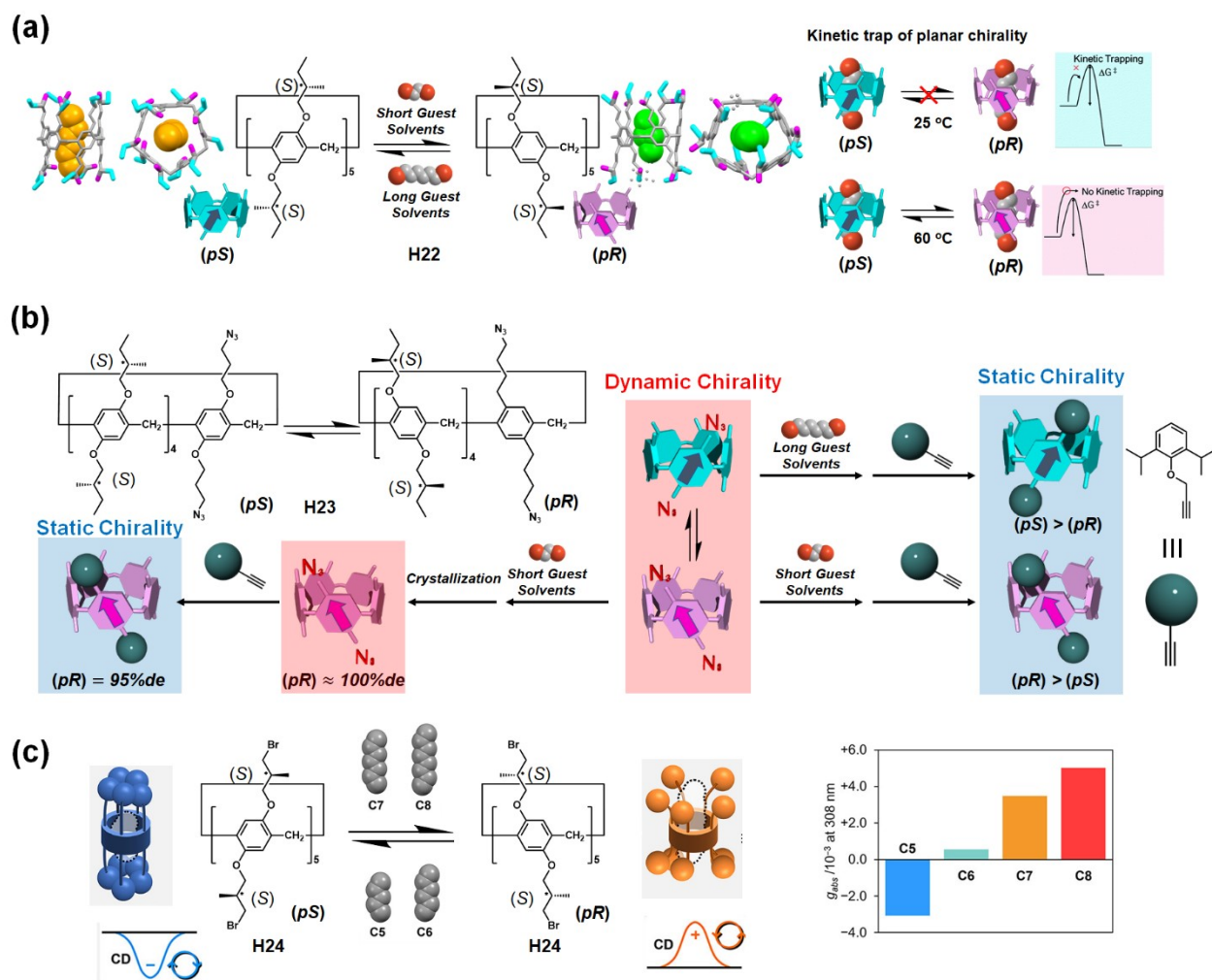
Figure 6. (a) Chemical structure of diastereomeric pillar[5]arene H22 and planar chiral inversion and holding by the achiral guest. Reproduced with permission from reference 118 (Copyright 2020 Royal Society of Chemistry). (b) Schematic representation of the planar chirality regulation and subsequent memory via introduction of covalent bonds. Reproduced with permission from reference 119 (Copyright 2023 Wiley-VCH Verlag GmbH & Co. KGaA). (c) Schematic representation of distinguishing n -alkane length with planar-chiral inversion. Reproduced with permission from reference 120 (Copyright 2023 American Chemical Society).
