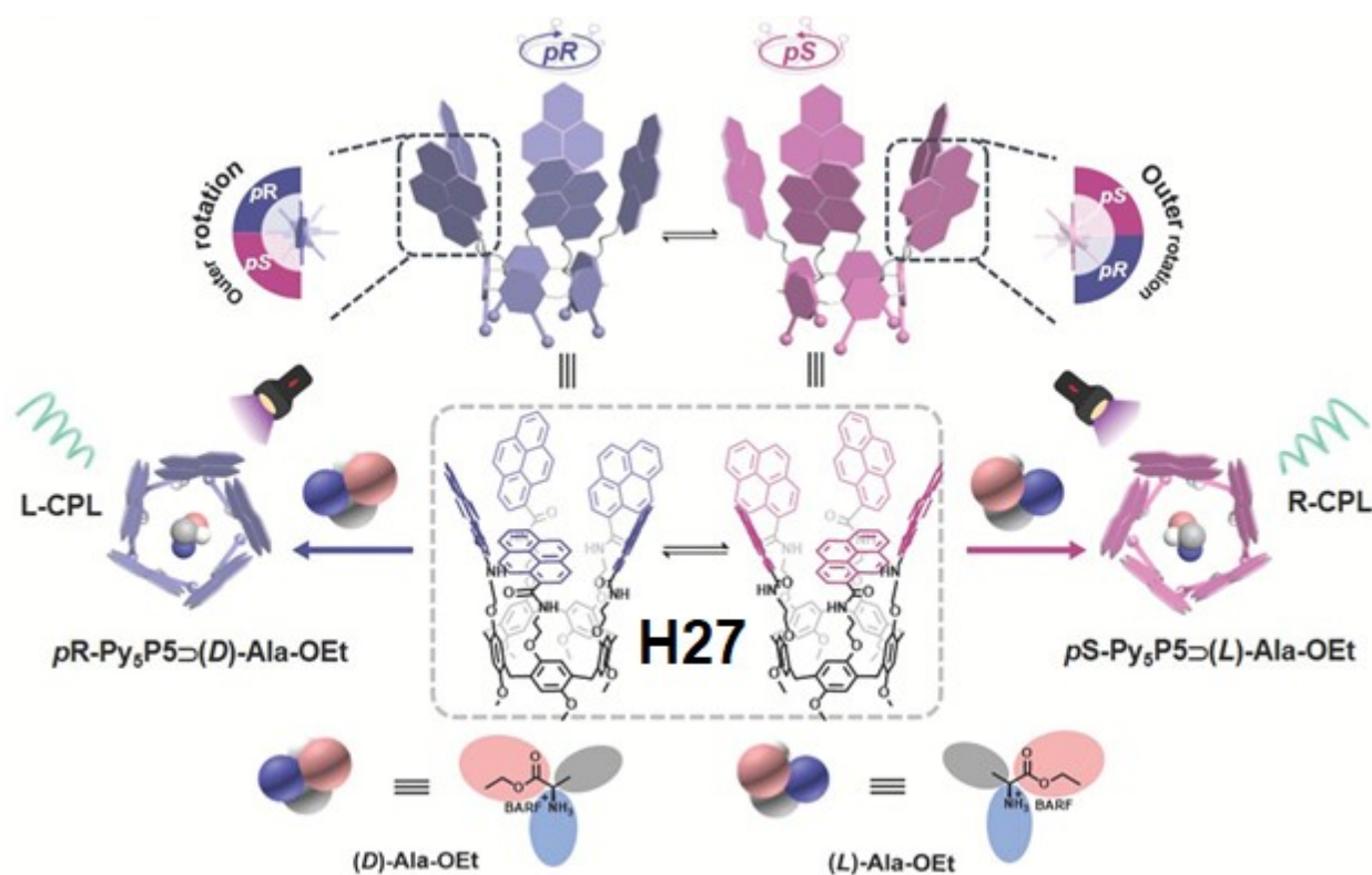
Figure 8. Schematic representation of the switching of left- and right-handed CPL by addition of chiral guests. Reproduced with permission from reference 137 (Copyright 2023 Wiley-VCH Verlag GmbH & Co. KGaA).
