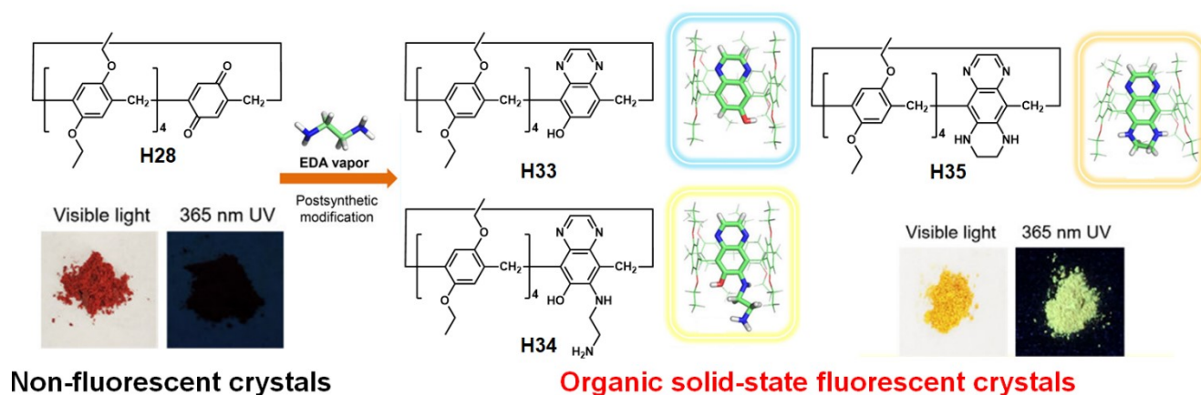
Figure 13. Schematic representation of the solid-vapor post-synthetic modification of H28 resulting in turn on vapoluminescence. Reproduced with permission from reference 148 (Copyright 2020 American Chemical Society).
