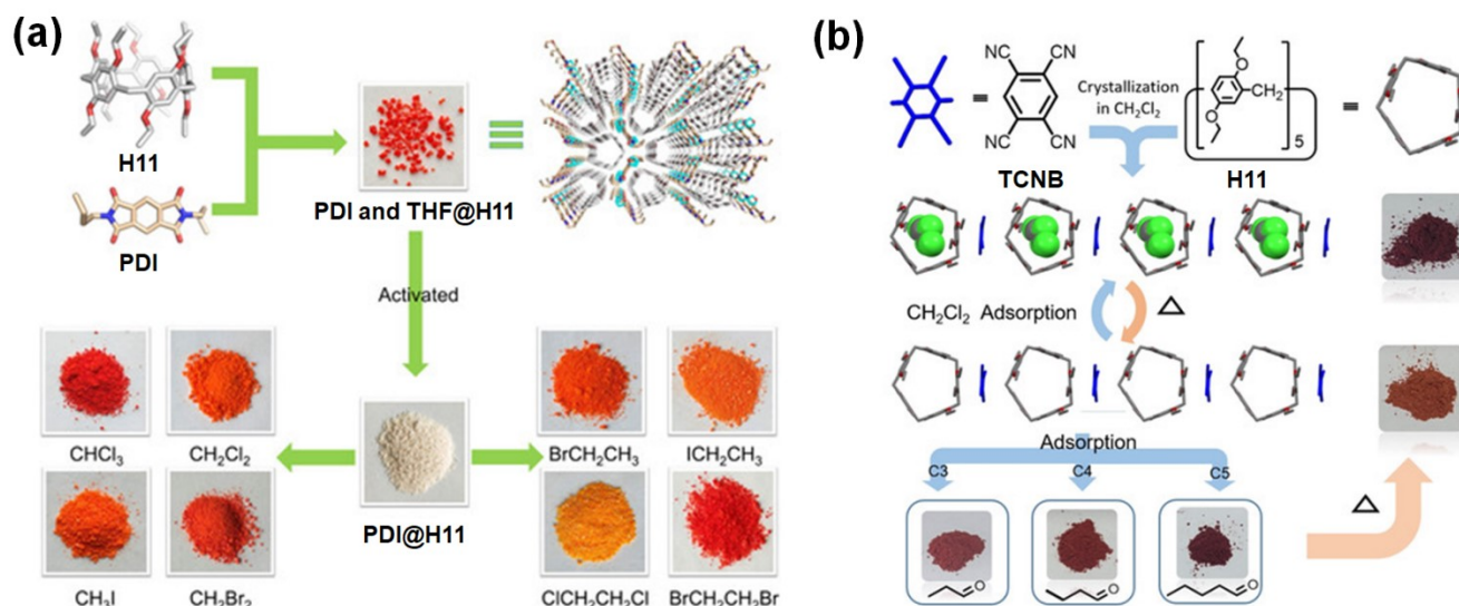
Figure 10. (a) Schematic representation of the vapochromism of cocrystals between H11 and PDI in response to haloalkane vapors. Reproduced with permission from reference 143 (Copyright 2020 Wiley-VCH Verlag GmbH & Co. KGaA). (b) Schematic representation of the vapochromism of cocrystals between H11 and TCNB in response to alkyl aldehyde vapor. Reproduced with permission from reference 144 (Copyright 2021 Wiley-VCH Verlag GmbH & Co. KGaA).
