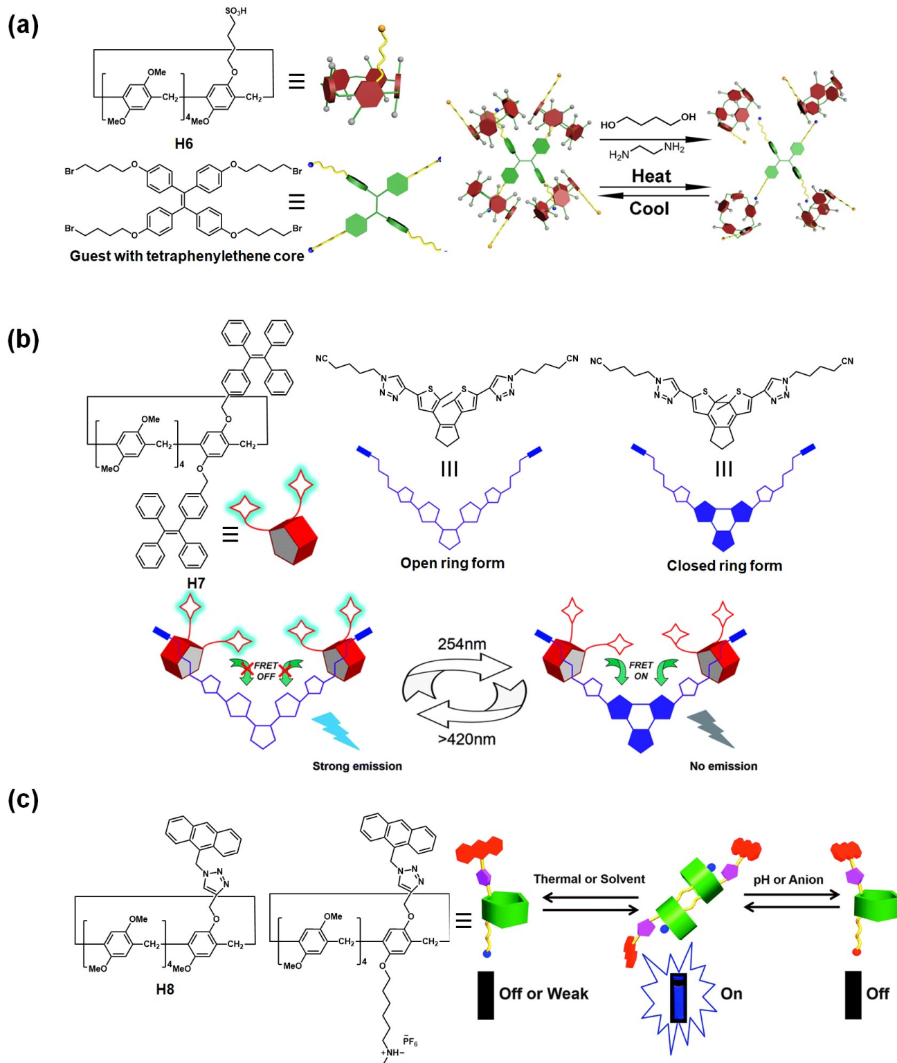
Figure 4. (a) Schematic representation of the pseudorotaxane formation between H6 and the tetraphenylethene derivative guest, and its response to stimuli. Reproduced with permission from reference 104 (copyright 2018 The Author(s) under the terms of the Creative Commons CC BY license.). (b) Schematic representation of the photoresponsive fluorescence switching of the pseudo[3]rotaxane between H7 and bithienylethene derivative guest. Reproduced with permission from reference 105 (Copyright 2018 Royal Society of Chemistry). (c) Schematic representation of the switching emission of the [c2]daisy chain under different external stimuli. Reproduced with permission from reference 106 (Copyright 2014 Royal Society of Chemistry).
