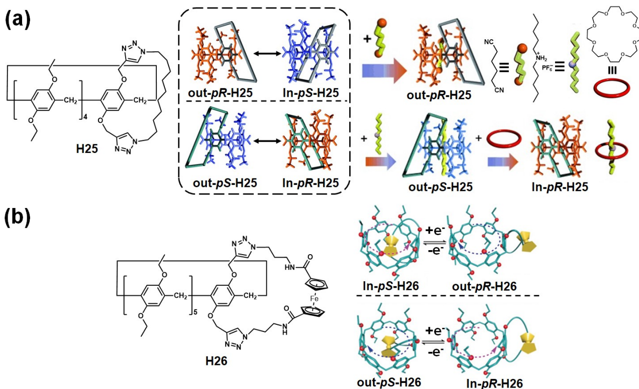
Figure 7. Planar chiral inversion based on pseudo[1]catenane of (a) pillar[5]arene and (b) pillar[6]arene. Reproduced with permission from references 121 and 122 (Copyright 2013 and 2020 Wiley-VCH Verlag GmbH & Co. KGaA).
