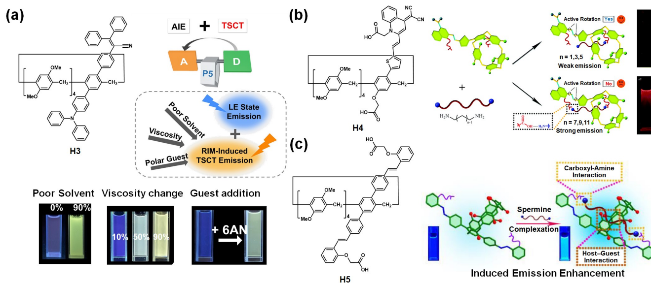
Figure 3. (a) Chemical structure of H3 exhibiting dual emission and fluorescence regulation triggered by poor solvent, viscosity change, and guest addition. Reproduced with permission from reference 89 (Copyright 2022 Wiley-VCH Verlag GmbH & Co. KGaA). Schematic representation of the fluorescence enhancement mechanism using three binding sites of (b) H4 and (c) H5 for detection of alkane diamines and spermine, respectively. Reproduced with permission from references 91 and 92 (Copyright 2020 Royal Society of Chemistry and 2023 Elsevier Inc).
