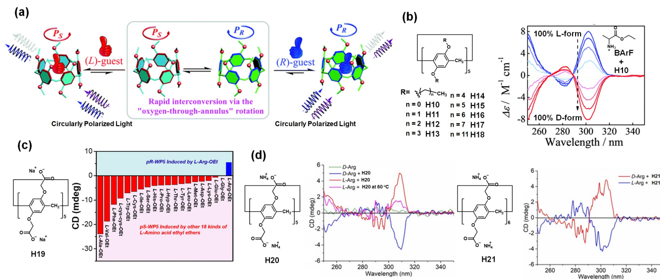
Figure 5. (a) Schematic representation of the planar chiral regulation by chiral guests. Reproduced with permission from reference 110 (Copyright 2020 Royal Society of Chemistry). Chemical structures and CD signal responses of (b) H10–H18, (c) H19, and (d) H20 and H21. Reproduced with permission from references 110, 111, and 112 (Copyright 2020 Royal Society of Chemistry, 2020 American Chemical Society, and 2020 Wiley-VCH Verlag GmbH & Co. KGaA).
