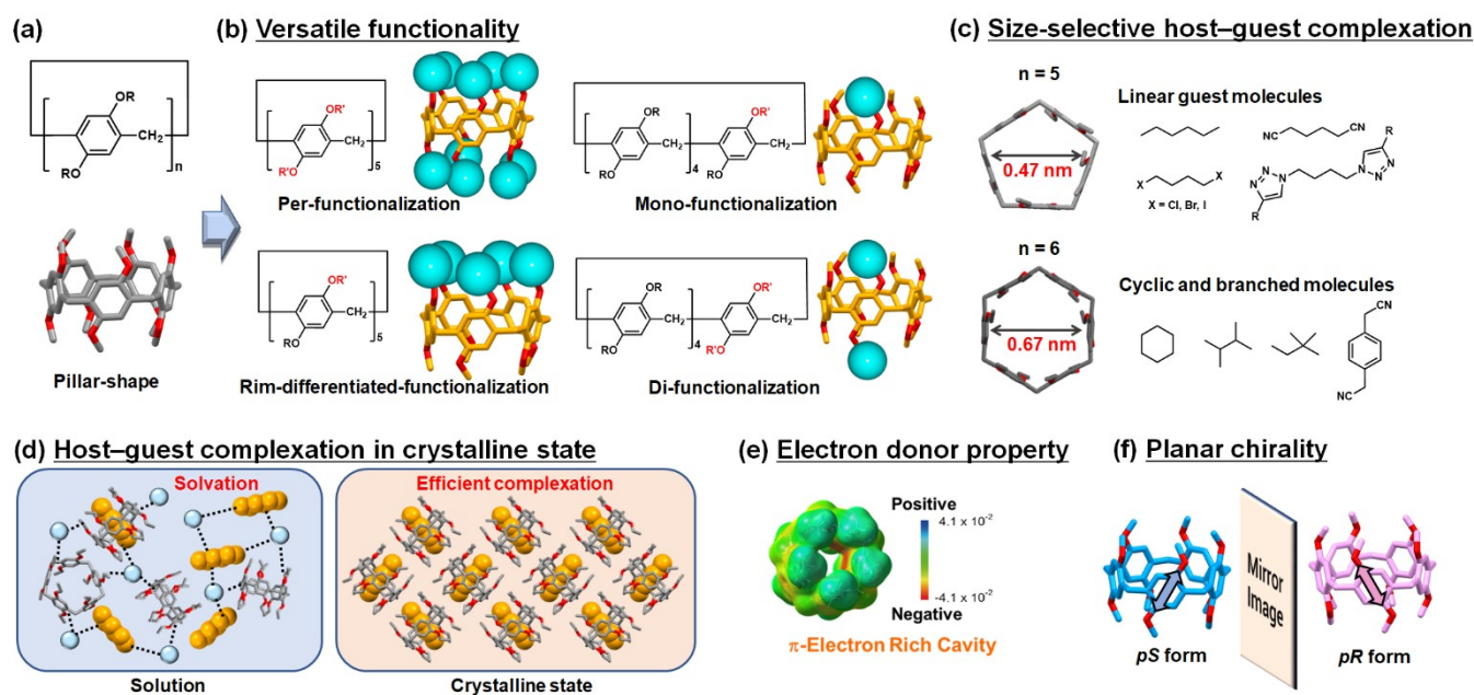
Figure 1. (a) Chemical and crystallographic structure of pillar[ n ]arene. (b) Versatile functionality of pillar[ n ]arene. (c) Cavity sizes of pillar[5]arene and pillar[6]arene, and suitable guest molecules for pillar[5]arene and pillar[6]arene. (d) Host-guest complexation events in solution and crystalline states. (e) Electrostatic potential profile of perethylated pillar[5]arene. (f) Planar chirality of pillar[ n ]arene.
