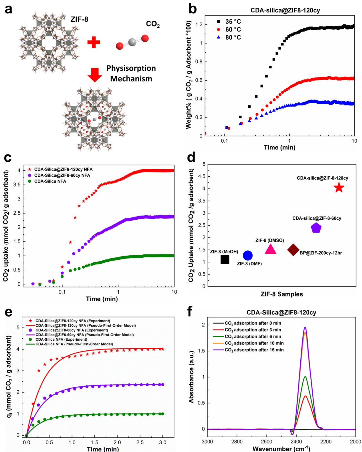
Figure 4. CO 2 adsorption capacity of CDA-silica@ZIF-8 NFA: a) schematic illustration of CO 2 adsorption in ZIF-8 through physisorption mechanism, b) CO 2 uptake of CDA-silica @ZIF8-
