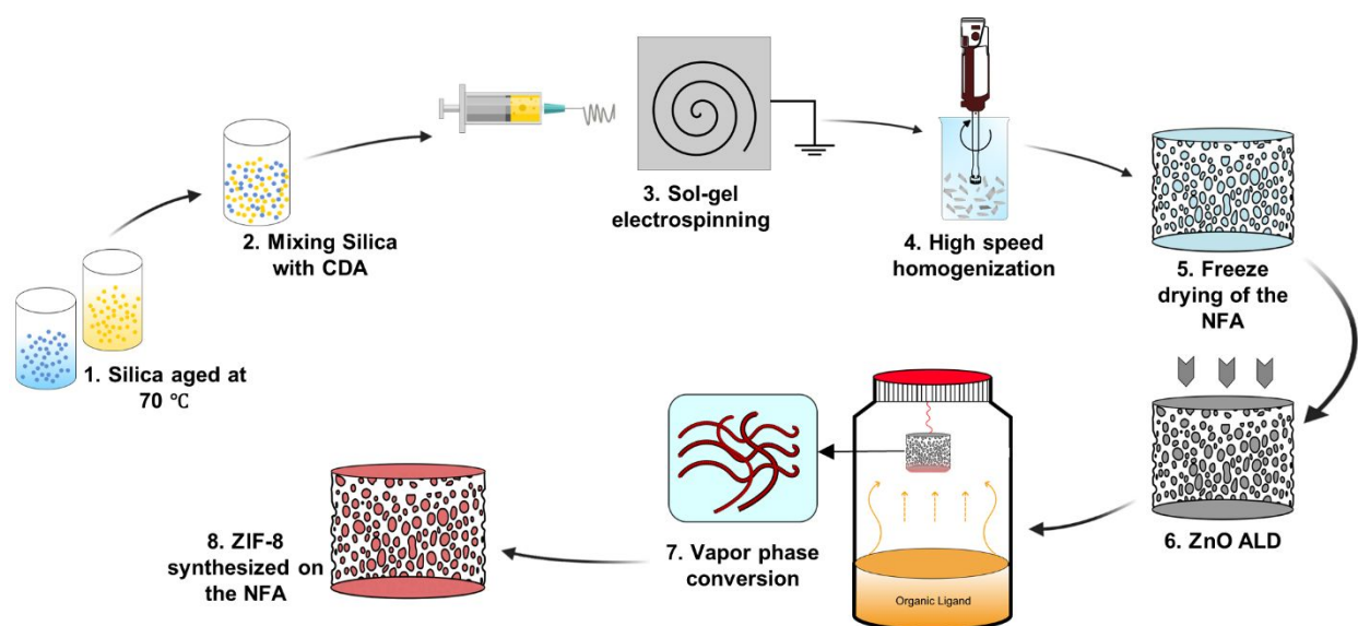
Figure 1. Pathway toward fabrication of CDA-silica@ZIF-8 NFA.
