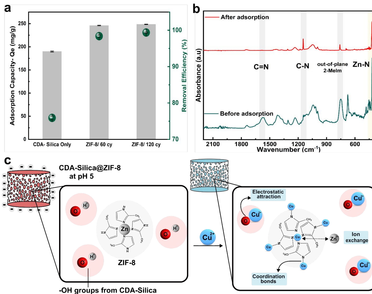
Figure 5. Heavy metal removal: a) adsorption capacity (mg/g) and removal efficiency (green circles, %) for 20 mg of the adsorbent (aerogel) load in 100 mg/L of stock solution of \text{Cu}^{2+} ions and b) FTIR spectra of CDA-Silica@ZIF-8/120cy before and after adsorption of \text{Cu}^{2+} . Note that all three samples in (a) are aerogels. (c) Adsorption mechanism depicting ion-exchange with Zn and coordination complex of Cu with N atoms of ZIF-8
