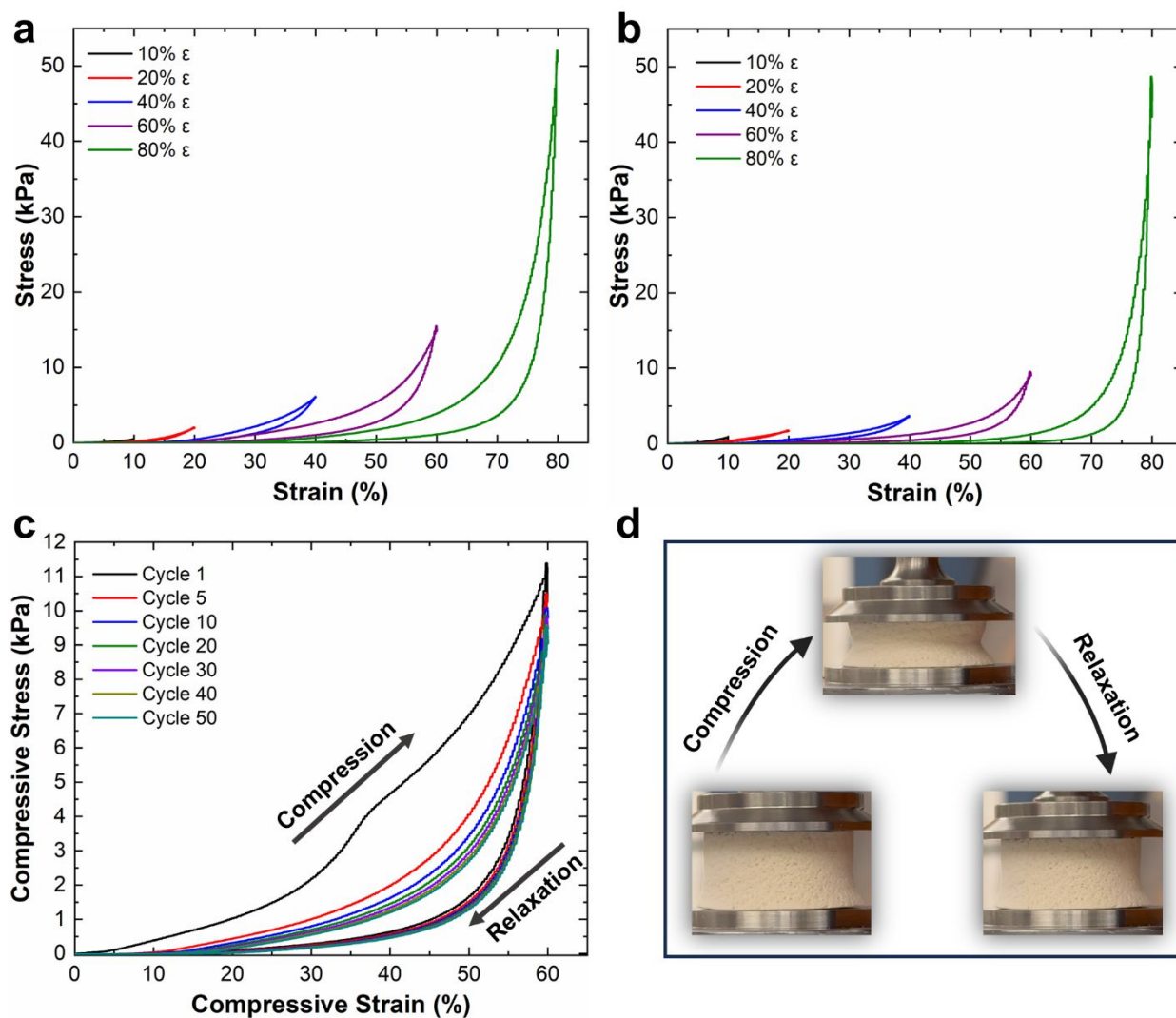
Figure 3. Compressive stress-strain experiments of a) CDA-silica NFA, b) CDA-silica@ZIF-8 NFA, c) cyclic fatigue test of CDA-silica@ZIF-8 NFA at 60% strain for 50 cycles and d) digital photograph of how the CDA-silica@ZIF-8 NFA changes under compressive deformation.
