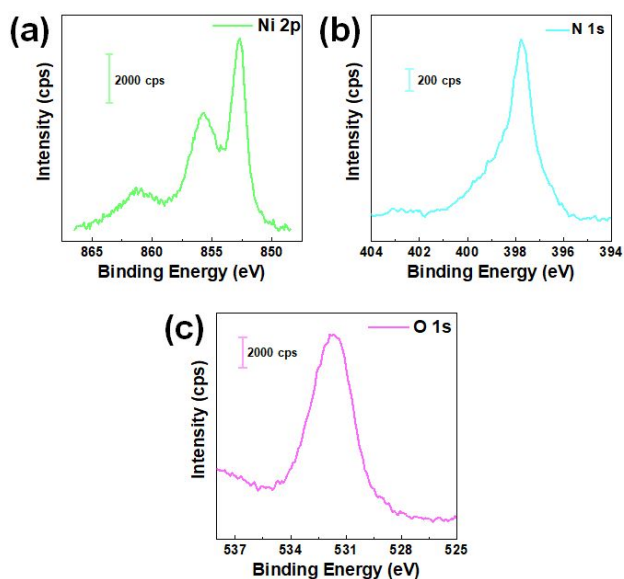
Fig. 4 (a) Ni 2p, (b) N 1s, and (c) O 1s XPS spectra of pristine Ni 3 N/NF.
