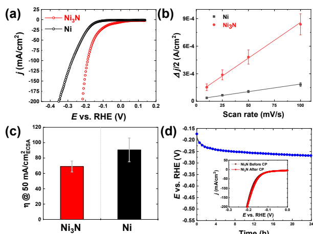
Fig. 5 (a) LSV curves, (b) double-layer capacitances ( C_{dl} ), and (c) ECSA-normalized HER overpotential values for Ni 3 N/NF and NF. (d) 24 h chronopotentiometry of Ni 3 N/NF at a constant current density of -20 mA/cm 2 .
