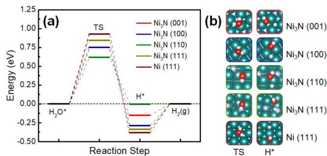
Fig. 6 (a) Calculated HER free energy pathways on Ni 3 N(001), Ni 3 N(100), Ni 3 N(110), Ni 3 N(111), and Ni(111) surfaces in alkaline media. (b) Modelled Ni-terminated Ni 3 N and Ni metal surfaces at two different states [i.e., transition state (TS) and H* adsorbed state]. Green, blue, red, and white spheres represent Ni, N, O, and H, respectively.
