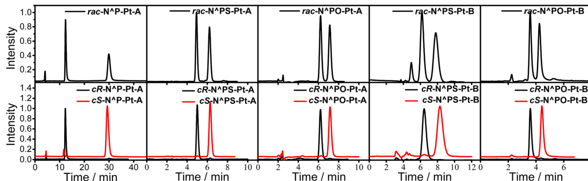
Fig. 2 Top: chiral HPLC traces of rac -N A -Pt-A, rac -N A PS-Pt-A, rac -N A PO-Pt-A, rac -N A PS-Pt-B, and rac -N A PO-Pt-B. Bottom: chiral HPLC traces of enantiopure ( cR ) (black line) and ( cS ) (red line) Pt(II) complexes.
