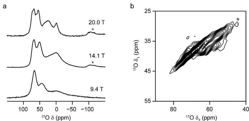
Fig. 2 ^{17}\text{O} NMR of \gamma\text{-Al}_2\text{O}_3 enriched by post-synthetic exchange with ^{17}\text{O}_2 (g). (a) MAS NMR spectra of \gamma\text{-Al}_2\text{O}_3 (500 °C), acquired at the magnetic fields shown. (b) ^{17}\text{O} (20.0 T, 30 kHz) DQF-STMAS 49 NMR spectrum of \gamma\text{-Al}_2\text{O}_3 (950 °C). For detailed experimental parameters see Section S1 of the ESI†
