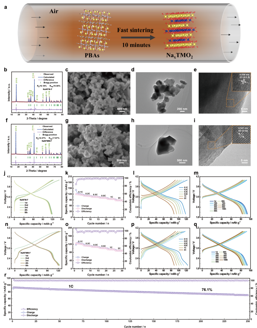
Fig. 4 (a) Schematic diagram of the transformation process from PBAs to layered oxides. (b) Powder XRD result with Rietveld refinement of NaNFMM-F. (c) SEM, (d) TEM, and (e) HRTEM images of NaNFMM-F. (f) Powder XRD result with Rietveld refinement of NaNFMM-F. (g) SEM image of NaNFMM-F. (h) TEM and (i) HRTEM images of NaNFMM-F. Electrochemical performance of the electrode within the potential window of 2–4 V: GCD curves at 0.1 C for (j) NaNFMM-F and (n) NaNFMM-F. Rate performance of (k) NaNFMM-F and (o) NaNFMM-F. GCD curves at different rates of (l) NaNFMM-F and (p) NaNFMM-F. GCD curves at different cycles of (m) NaNFMM-F and (q) NaNFMM-F. (r) Cycling performance of NaNFMM-F.
