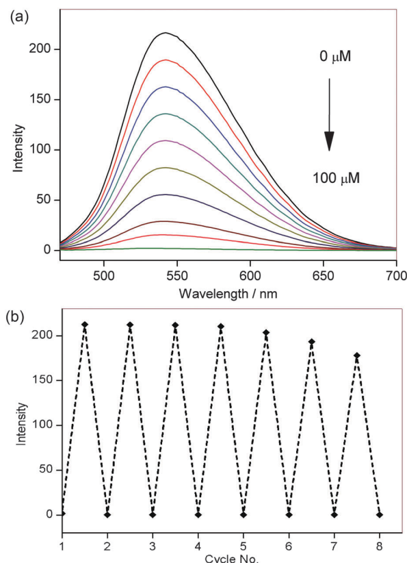
Fig. 2 Photophysical behaviour of NpFR1. (a) Fluorescence emission of NpFR1 (5 \mu M, \lambda_{\text{ex}} = 405 nm) with the incremental addition of sodium dithionite. (b) Fluorescence response of NpFR1 to cycles of oxidation and reduction. Reduction was achieved with sodium dithionite (100 \mu M) followed by re-oxidation with 250 \mu M \text{H}_2\text{O}_2 . Spectra were recorded 5 min after the addition of reducing and oxidising agents. All spectra were acquired in HEPES buffer (100 mM, pH 7.4).
