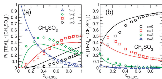
Fig. 15 Percentage of methylsulfonate- (a) and triflate-ions (b) hydrogen-bonded to zero, one, two, and three TEA-cations as a function of the mixture-composition at 400 K. Symbols: MD-simulation. Solid lines: model using equal statistical weights with w_{6,n} = 1 for n \leq 3 and w_{6,n} = 0 for n > 3 .
