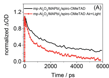
Fig. 5 Time-resolved transient absorption at 780 \text{ nm} for pristine mp- \text{Al}_2\text{O}_3/\text{MAPbI}_3/\text{spiro-OMeTAD} (black) and exposed to air and ambient light \text{MAPbI}_3/\text{spiro-OMeTAD} (red) films. Traces normalized to \Delta OD = 1 at 1 \text{ ps} time-delay to highlight differences in recombination kinetics. Laser excitation energy density = 25 \mu\text{J cm}^{-2} at 567 \text{ nm} .
