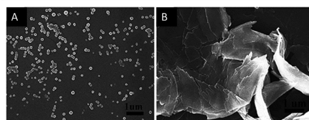
Fig. 34 Schematic representation of the anion- \pi induced self-assembly forming the vesicle as well as SEM images before (A) and after addition of 3 eq. of \text{NaNO}_3 (B). Reproduced with permission from John Wiley and Sons. 66
