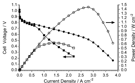
Fig. 13 The AEMFC performances at 80^\circ\text{C} of the LDPE-AEM (100 kGy) with \text{O}_2 (●, ○) and \text{CO}_2 -free air (■, □) supplies as the cathode: PtRu/C (50% wt Pt and 25% wt Ru) anodes and Pt/C (40% wt) cathodes (all 0.4\text{ mg}_{\text{Pt}}\text{ cm}^{-2} loadings). The 1.0 SLPM (RH = 100%) cathode and anode ( \text{H}_2 ) gas supplies were not pressurised.
