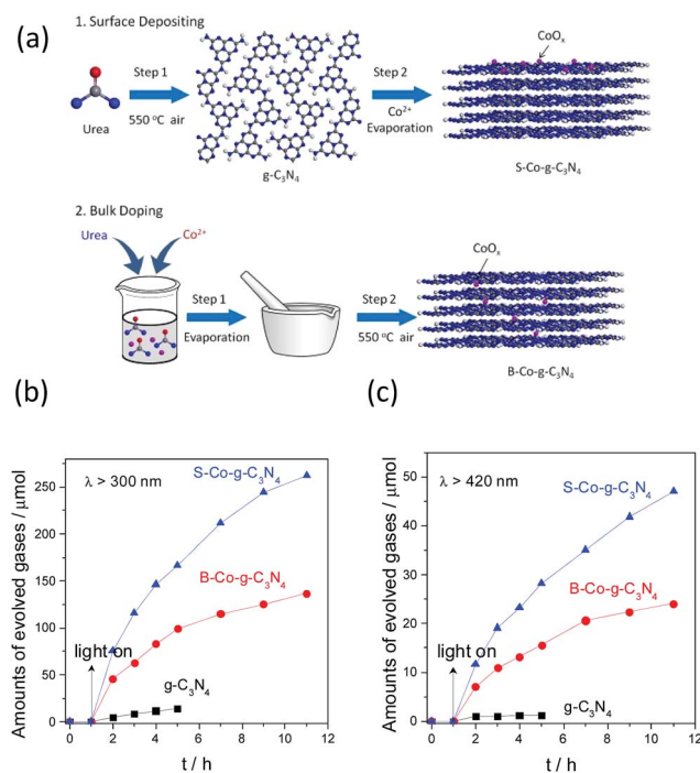
Fig. 11 (a) Schematic illustration of surface modification and bulk doping modification of \text{g-C}_3\text{N}_4 . Photocatalytic water oxidation activities of the \text{g-C}_3\text{N}_4 , B-Co-g- \text{C}_3\text{N}_4 and S-Co-g- \text{C}_3\text{N}_4 samples under (b) UV ( \lambda > 300 \text{ nm} ) and (c) visible light ( \lambda > 420 \text{ nm} ) irradiation. Reprinted with permission from ref. 107. Copyright 2016, American Chemical Society.
