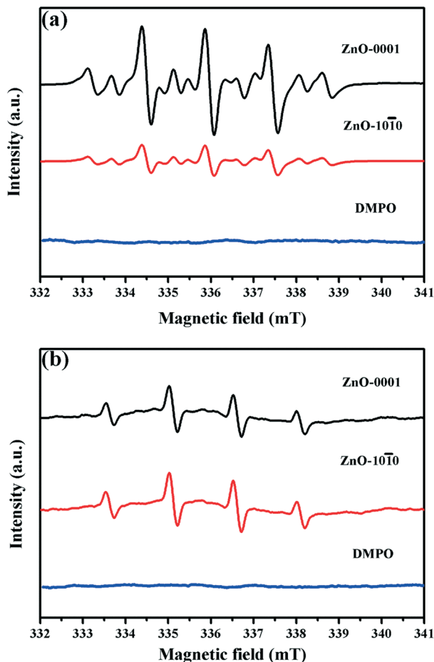
Fig. 4 EPR spectra of the ZnO nanomaterials ( 1.2 \times 10^{-2} \text{ mol L}^{-1} ) and DMPO ( 0.25 \text{ mol L}^{-1} ) in (a) methanolic and (b) aqueous suspensions after irradiation by simulated solar light.
