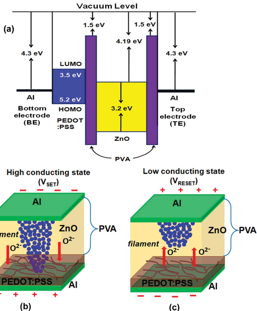
Fig. 5 Schematic diagrams of energy level corresponding to the operating mechanism for the S3 memory device. Schematic diagrams of the electronic structures corresponding to the operating mechanisms for S3 memory device with the (b) high conducting state (SET state) and the (c) low conducting state (RESET state).
