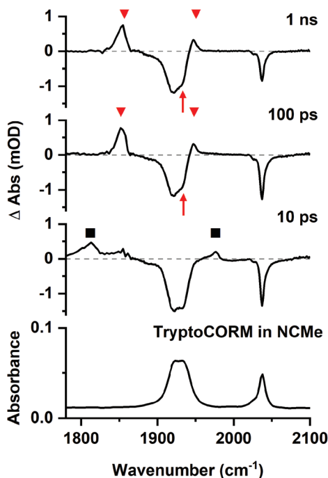
Fig. 3 Bottom IR spectrum of trypto-CORM in NCMe in the region 1780–2100 cm -1 . Top time-resolved difference IR spectra for the photolysis (400 nm) of trypto-CORM in NCMe with pump-probe delays of 10 ps, 100 ps, and 1 ns showing bands for A and B (■) and C by (▼). The red arrows show the apparent recovery of the GSB for trypto-CORM.
