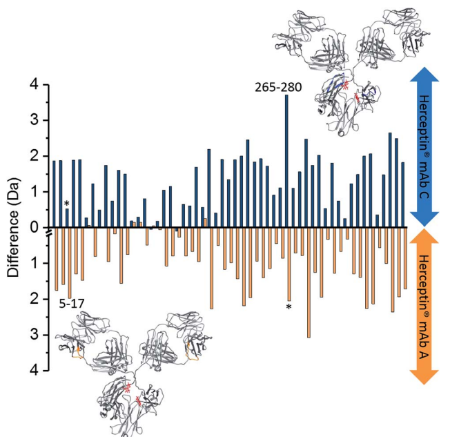
Fig. 4 Deuterium uptake difference plots for heavy chain (HC) intact vs. endoS2 treated Herceptin®; endoS2–intact. Each bar represents a different peptide (HC sequence coverage = 70.2%, 55 peptides). Blue bars represent the deuterium uptake differences for Herceptin® lot C; orange bars represent deuterium uptake differences for Herceptin® lot A. Labelled peptides 5–17 (VESGGGLVQPGGS) and 265–280 (VVVDVSHEDPEVKFNW) are those with significant uptake differences between the two Herceptin® lots i.e. a difference of >1 Da (see ESI Fig. S16† for the Herceptin® lot C–lot A subtraction plot); * corresponds to the equivalent peptide in the other sample. The peptide locations for the two peptides with uptake differences >1 Da are highlighted on the mAb structures in blue and orange for lot C and lot A, respectively (PDB: 1IGY). A representation of endoS2 treated glycans are shown in red. Subtraction of intact mAb data from enzyme treated mAb data for individual lots, means that the intact data serves as a control to counteract any day-to-day variations in the HDX setup. An interactive version of this figure is available at the following link; http://bit.ly/2OjV3R6 .
