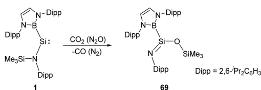
Scheme 26 Activation of \text{N}_2\text{O} and \text{CO}_2 by the acyclic silylene 1 .
