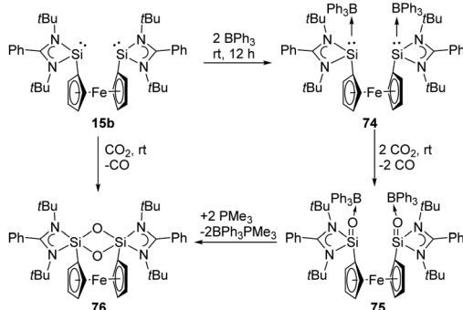
Scheme 27 Activation of \text{N}_2\text{O} and \text{CO}_2 by Lewis acid/base-stabilised \text{Si}^{\text{II}} species 70 , 72a, b , 15b and 74 .
