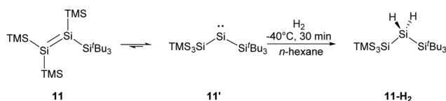
Scheme 7 Activation of H 2 by a mixture of tetrasilyldisilene 11 and bis(silyl)silylene 11' .
