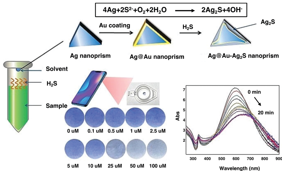
Fig. 17 Biosafety materials for food safety. Schematic illustration of the H 2 S sensing mechanism based on the Ag@Au core-shell nanoprobe. Reproduced with permission from ref. 204. Copyright 2019, American Chemical Society.
