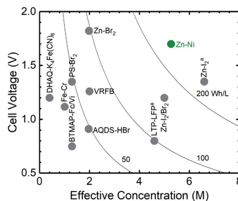
Fig. 1 Theoretical volume energy densities of some representative aqueous flow battery chemistries including VRFB, 11 Fe–Cr, 33 BTMAP-Fc/Vi, 16 Zn–Br 2 , 34 LTP–LFP 3,4 , Zn–I 2 /Br 2 , 35 Zn–I 2 a , 39 PS–Br 2 (ref. 36) and DHAQ– \text{K}_4\text{Fe}(\text{CN})_6 , 14 and AQDS–HBr. 9 Abbreviations: BTMAP-Fc: 1,1'-bis[3-(trimethylammonio)propyl]ferrocene dichloride, BTMAP-Vi: bis[3-(trimethylammonio)propyl]viologen tetrachloride, PS: polysulfide, AQDS: 9,10-antraquinone-2,7-disulphonic acid, DHAQ: 2,6-dihydroxyanthraquinone, LTP: \text{LiTi}_2(\text{PO}_4)_3 , LFP: \text{LiFePO}_4 .
