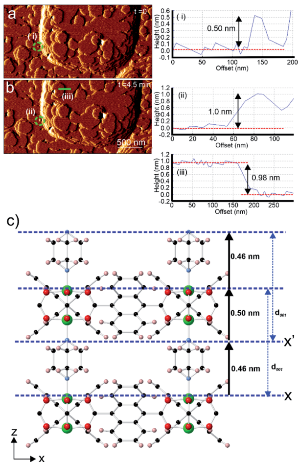
Fig. 3 In situ AFM deflection images of 1 with cross-section analyses showing the developing 2D nuclei (encircled by dotted green circles in (a) and b)). Crystal structure of 1 (c) displaying the various vertical heights of certain structural components above the possible surface terminating planes X and X'. AFM image size is 3.0 \times 1.5 \mu\text{m}^2 .
