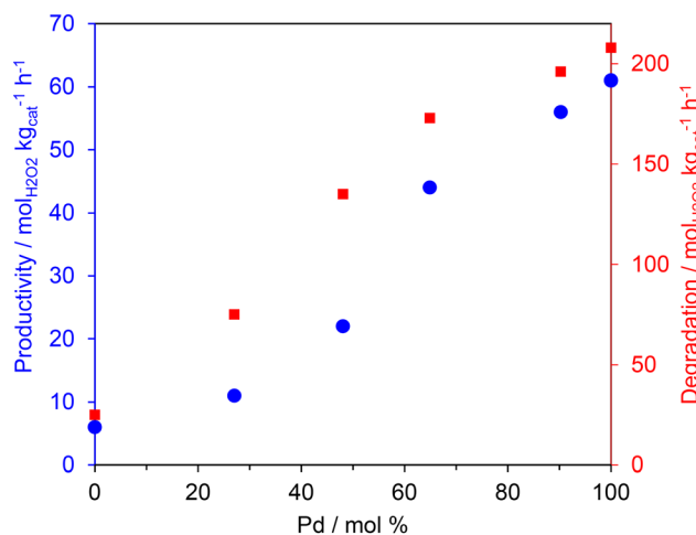
Fig. 1 The effect of Pd: Au ratio on the catalytic activity of 0.66%PdAu/TS-1 catalysts towards the direct synthesis (●) and subsequent degradation (■) of \text{H}_2\text{O}_2 . \text{H}_2\text{O}_2 direct synthesis reaction conditions: catalyst (0.01 g), \text{H}_2\text{O} (2.9 g), MeOH (5.6 g), 5% \text{H}_2/\text{CO}_2 (420 psi), 25% \text{O}_2/\text{CO}_2 (160 psi), 0.5 h, 2 °C, 1200 rpm. \text{H}_2\text{O}_2 degradation reaction conditions: catalyst (0.01 g), \text{H}_2\text{O}_2 (50 wt% 0.68 g), \text{H}_2\text{O} (2.22 g), MeOH (5.6 g), 5% \text{H}_2/\text{CO}_2 (420 psi), 0.5 h, 2 °C, 1200 rpm.
