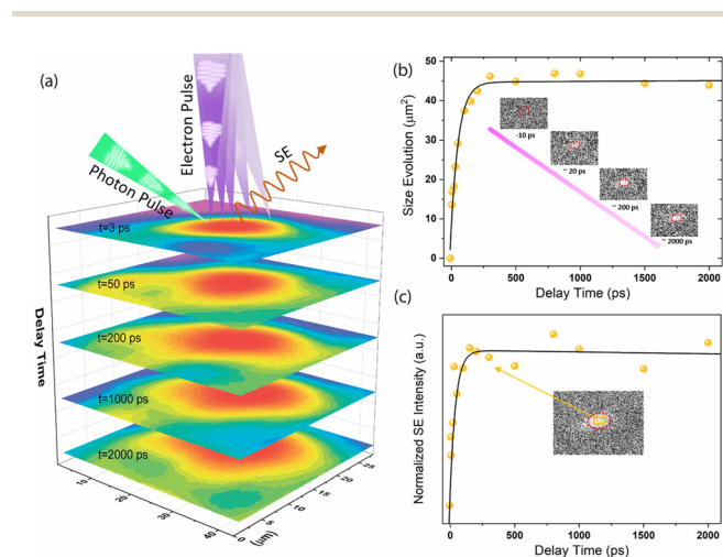
Fig. 4 (a) Color-coded ultrafast SEM images after photoexcitation. The transient images were obtained at different delay times and diffusion distances. The upper part of the images shows a simplified diagram of the time-resolved SEM process. In this process, the MAPbBr 3 crystal was excited by a photon pulse with repetition rate of 6.25 MHz. The probe electron pulses were generated by focusing the UV photon pulses onto the tip of the gun source, and the secondary electrons that escaped from the surface were collected by the SE detector. The images were fitted with a 2D Gaussian function to increase the signal-to-noise ratio. (b) Pump-induced spot size evolution on the sample surface as a function of the delay time between the photon pump and the electron probe. The inset shows the transient SEM images obtained at different delay times after photoexcitation. The red dashed circles represent the pump footprint. (c) Normalized SE intensity changes with the delay time. The intensities were normalized by rescaling the maximum value of the data matrix to 1 and were calculated by summing the intensities in a selected square at the centre of the beam spot (see the inset, orange rectangle area).
