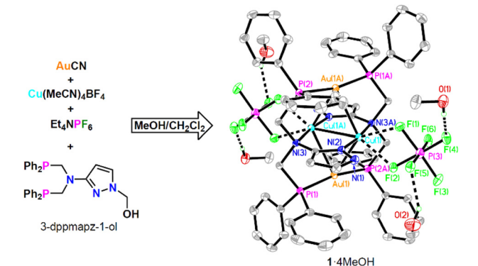
Fig. 1 Synthesis and crystal structure of 1 ·4MeOH with 50% thermal ellipsoids. All H atoms except for those of the H-bonded O–H groups are omitted for clarity. Symmetry codes for A: 1 – x, 1 – y, 1 – z; B: 1 – x, –y, 1 – z.
