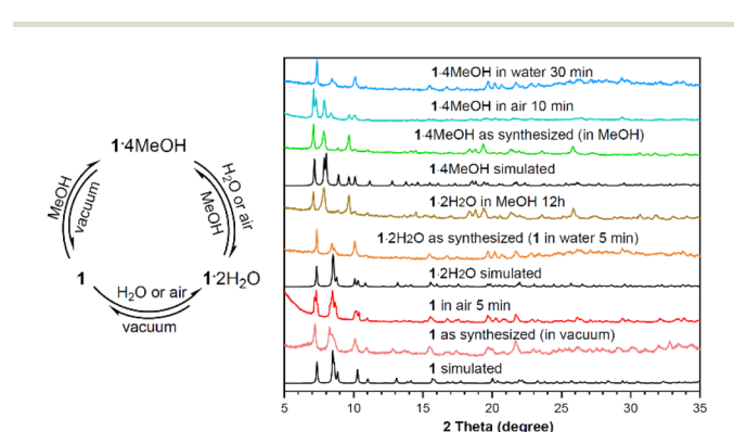
Fig. 2 Reversible inter-conversions of 1 , 1 ·2H 2 O and 1 ·4MeOH, with PXRD patterns simulated from the SCXRD data and those of the samples during the inter-transformations.
