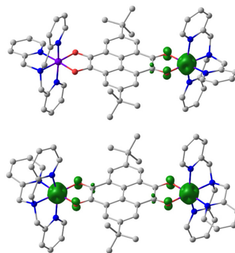
Fig. 9 Spatial structure and spin density distribution (contour value = 0.03 \text{e \AA}^{-3} ) of compound 3 in the \{\text{Co}^{\text{III-LS}}(\text{tpa})\text{-pyrene}^{\text{Cat-Sq-CO}^{\text{II-HS}}(\text{tpa})}\} (top) and \{\text{Co}^{\text{II-HS}}(\text{tpa})\text{-pyrene}^{\text{Sq-Sq-CO}^{\text{II-HS}}(\text{tpa})}\} (bottom) charge distributions, as calculated by the DFT UTPSSH/6-311++G(d,p) method. Hydrogen atoms and counter-ions are omitted for clarity.
