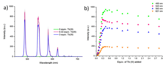
Fig. 4 (a) The overall changes to the \text{Tb}(\text{III}) -centred emission upon titrating 3 ( 1 \times 10^{-5} \text{ M} ) against \text{Tb}(\text{CF}_3\text{SO}_3)_3 (0 \rightarrow 3 equiv.) in \text{CH}_3\text{CN} at 22 \text{ }^\circ\text{C} . (b) The corresponding experimental binding isotherms for the \text{Tb}(\text{III}) emission at \lambda = 490, 545, 583 and 621 \text{ nm} . These results were fully reproducible (see enlarged version in ESI † ).
