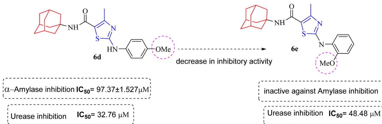
Fig. 8 Structural variation from 6d to 6e showing decrease in amylase and urease inhibitory action.
