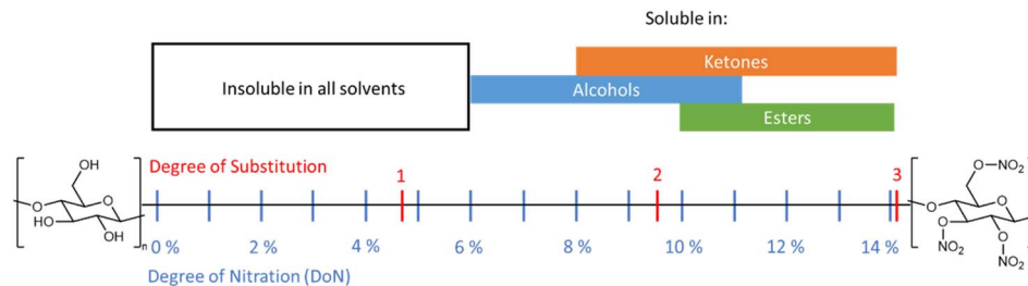
Fig. 11 Schematic summarising the solubility of NC across a variety of functional groups in relation to DoN. Solubility data from ref. 77.
