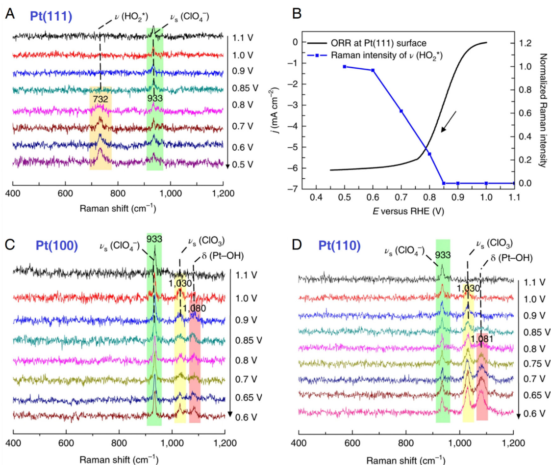
Fig. 12 (A) In situ EC-SHINERS spectra on the Pt(111) electrode in O_2 -saturated 0.1\text{ M HClO}_4 . (B) Potential-dependent Raman intensity of HO_2^* species on Pt(111) versus ORR current. ORR current was obtained in a O_2 -saturated 0.1\text{ M HClO}_4 solution using a rotating disk electrode Pt(111) electrode with a rotation rate of 1600 rpm. and a scan rate of 50\text{ mV s}^{-1} . (C) and (D) In situ EC-SHINERS spectra on Pt(100) (C) and Pt(110) (D) electrodes in O_2 -saturated 0.1\text{ M HClO}_4 . Reproduced with permission from ref. 146. Copyright 2018 Springer Nature.
