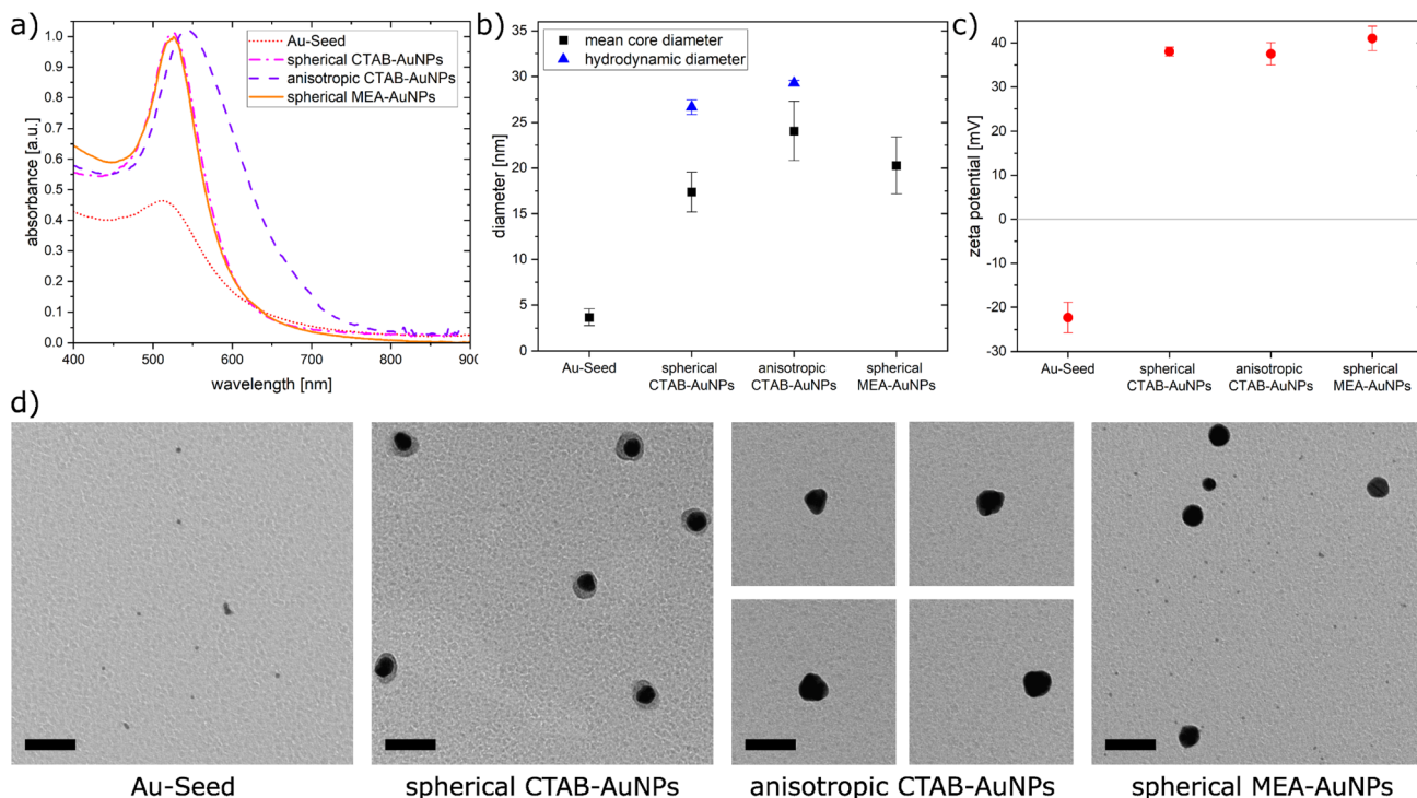
Fig. 2 (a) The absorbance spectra of the synthesized nanoparticles (b) calculated mean core diameter from the TEM images and hydrodynamic diameter measured by dynamic light scattering. (c) plot of the zeta potential for the synthesized nanoparticles, and (d) TEM images of synthesized gold nanoparticles. Scale bar is 50 nm.
