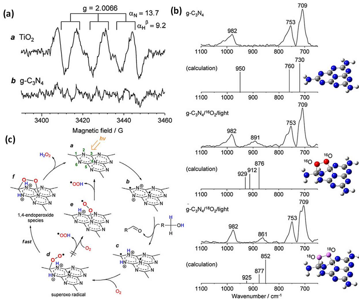
Fig. 23 (a) ESR spectra of solutions resulting from the photoillumination of \text{TiO}_2 and g\text{-C}_3\text{N}_4 in an ethanol/water/ \text{O}_2 system. (b) Raman spectra and calculated Raman shifts for g\text{-C}_3\text{N}_4 following photoreaction with ^{16}\text{O}_2 and ^{18}\text{O}_2 in an ethanol/water mixture. (c) The mechanism for the selective formation of \text{H}_2\text{O}_2 on g\text{-C}_3\text{N}_4 under visible light illumination. The figures are reproduced with permission from ref. 66. Copyright 2023, Wiley-VCH.
