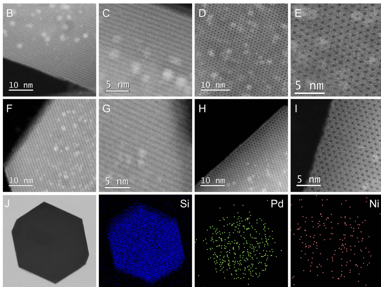
Fig. 1 (A) Schematic illustration of the preparation of zeolite-encaged Pd-based catalysts. C_e -corrected STEM images of (B and C) Pd@S-1-C; (D and E) 0.8Pd0.2Ni(OH) 2 @S-1-C; (F and G) Pd@S-1-H; (H and I) 0.8Pd0.2Ni(OH) 2 @S-1-H. (J) TEM image of 0.8Pd0.2Ni(OH) 2 @S-1-H catalyst and corresponding EDX mapping images for Si, Pd, and Ni elements. Scale bar: 250 nm.
