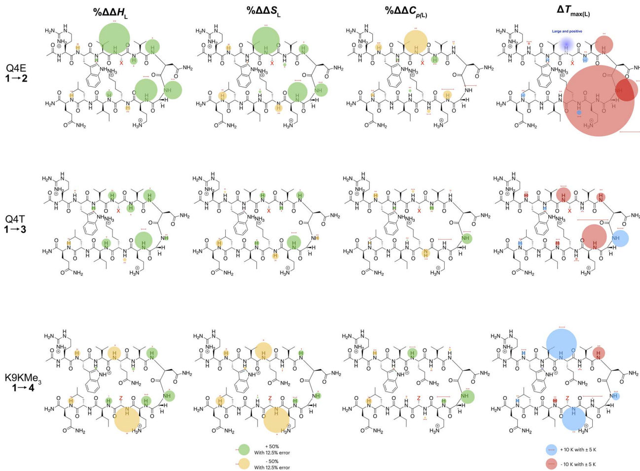
Fig. 4 Per-residue reporting of the \% \Delta \Delta H_L , \% \Delta \Delta S_L and \% \Delta \Delta C_{p(L)} and \Delta T_{\max(L)} for unfolding of the mutations: top row, Q4E (1 → 2); middle row, Q4T (1 → 3), and; bottom row, K9KMe 3 (1 → 4). Because of signal overlap between each peptide and its reference 6-mer half peptide, data could not be obtained for R1 and L11. For the \Delta H_L , \Delta S_L and \Delta C_{p(L)} data, changes are shown as percentage increases (green) or decreases (yellow) proportional to the area of the bubble. For \Delta T_{\max(L)} , changes are shown in kelvin (K). All values are indicated, though bubbles for insignificant changes may not be apparent. Scaling bubbles and error bars for the two types of bubbles are shown at the foot of the figure. Specific values of \Delta H_L , \Delta S_L and \Delta C_{p(L)} as reported by each amide N–H are given in Fig. 3.
