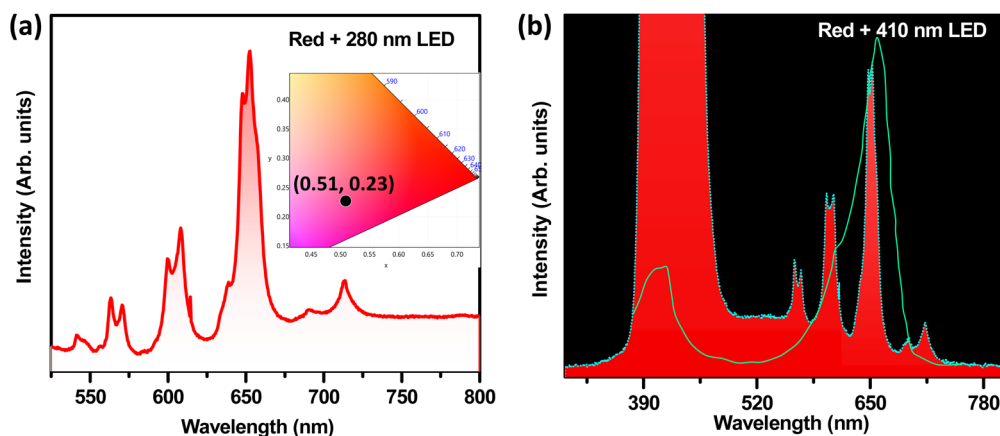
Fig. 10 (a) The electroluminescence spectra for the Sc 2 Mo 3 O 12 :Sm 3+ sample excited with 280 nm LED. The inset shows the chromaticity diagram for the same sample showing the CIE coordinates. (b) The electroluminescence spectra for the Sc 2 Mo 3 O 12 :Sm 3+ sample excited with 410 nm LED, along with the absorption spectra of the plant pigment phytochrome P R .
